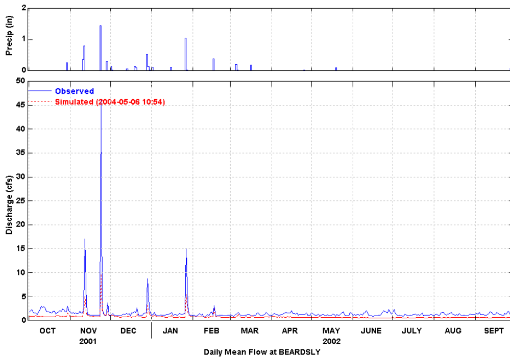
Figure 14 Simulated and Observed Daily Flow at Beardsley (WY 2002)
