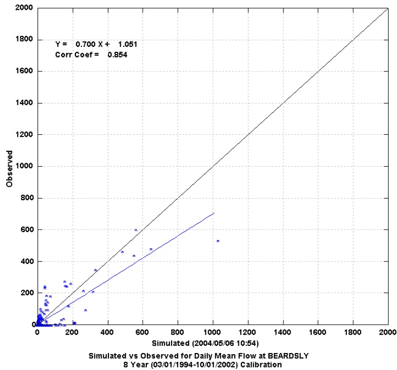
Figure 2 Daily Scatter Plot of Simulated versus Observed Flow at Beardsley
