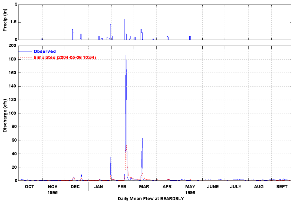
Figure 8 Simulated and Observed Daily Flow at Beardsley (WY 1996)
