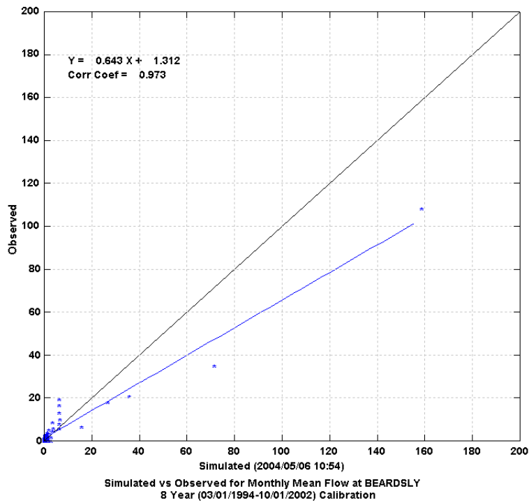
Figure 3 Monthly Scatter Plot of Simulated versus Observed Flow at Beardsley
