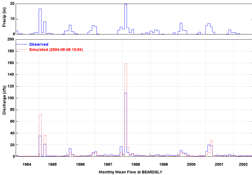
Figure 5 Simulated and Observed Monthly Flow at Beardsley (WY 1994-2002)
