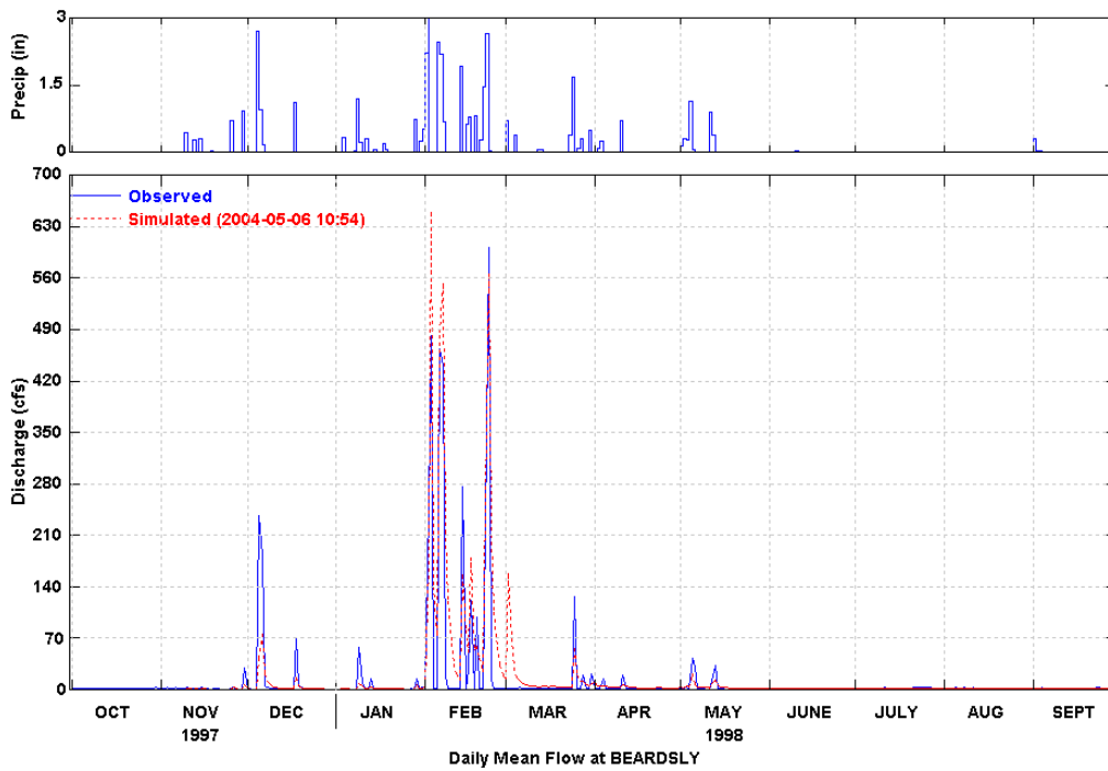
Figure 10 Simulated and Observed Daily Flow at Beardsley (WY 1998)
