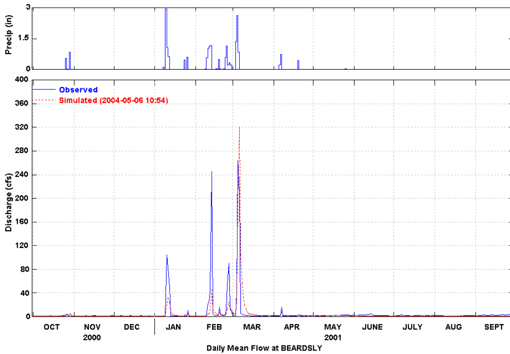
Figure 13 Simulated and Observed Daily Flow at Beardsley (WY 2001)
