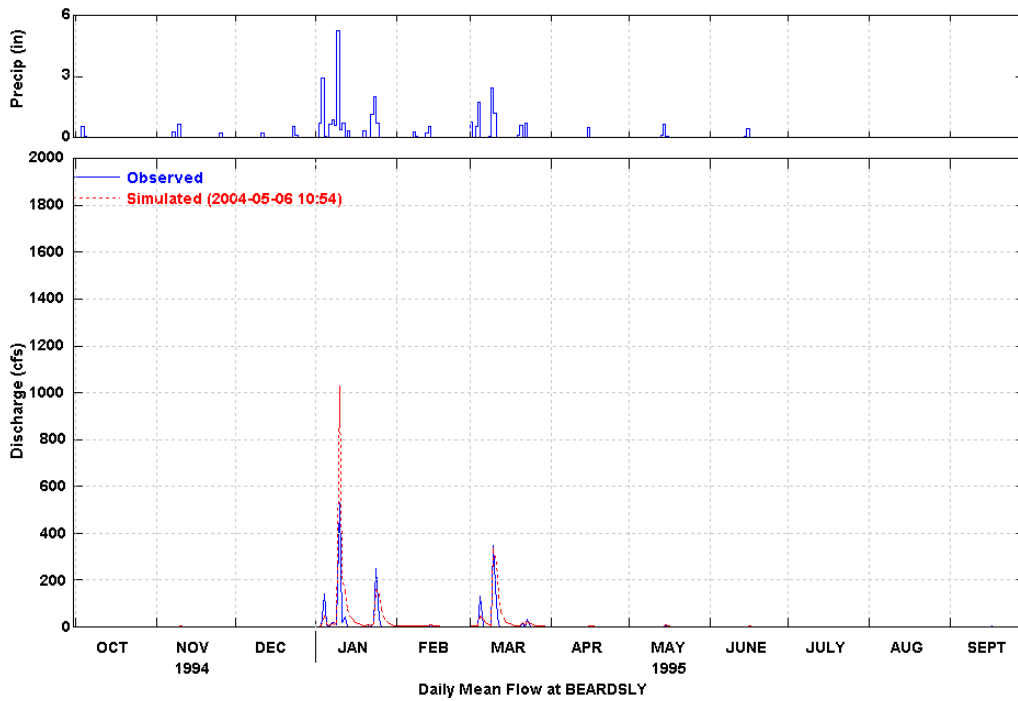
Figure 7 Simulated and Observed Daily Flow at Beardsley (WY 1995)
