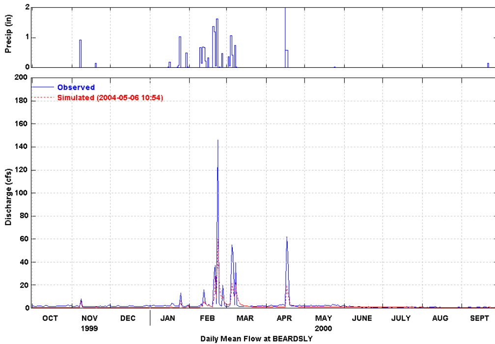
Figure 12 Simulated and Observed Daily Flow at Beardsley (WY 2000)
