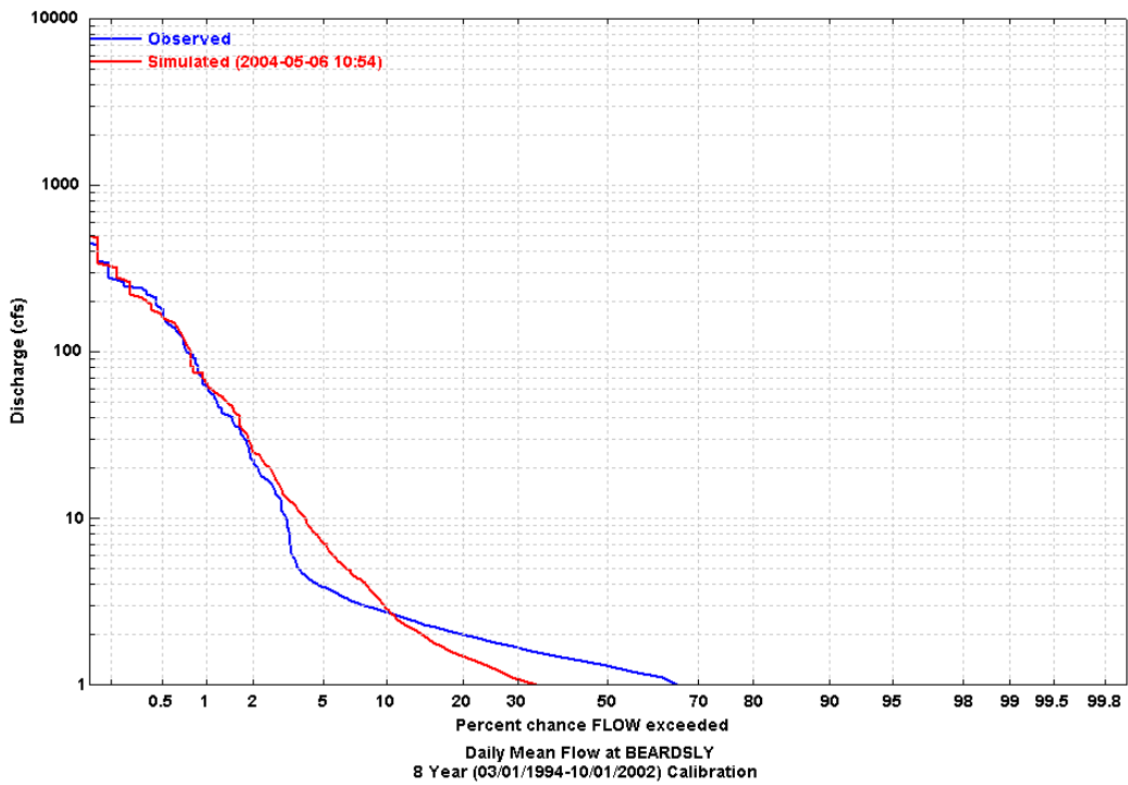
Figure 1 Simulated and Observed Daily Flow Duration Curve at Beardsley
