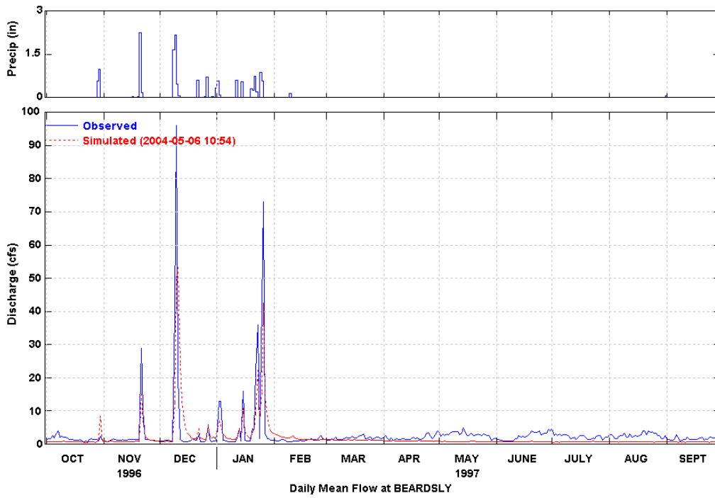
Figure 9 Simulated and Observed Daily Flow at Beardsley (WY 1997)
