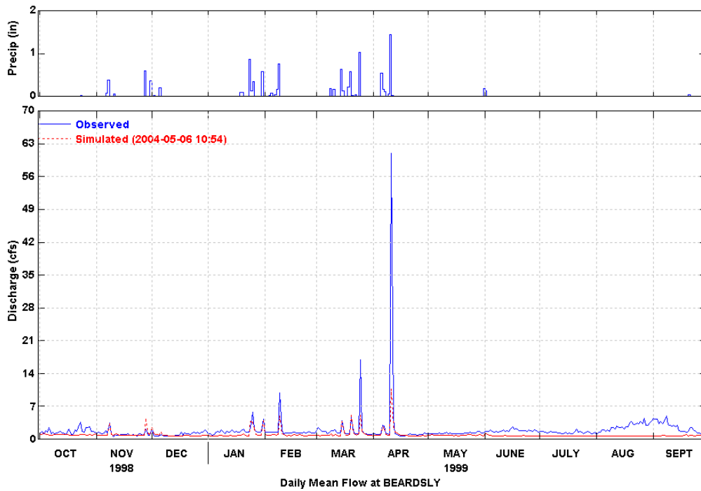
Figure 11 Simulated and Observed Daily Flow at Beardsley (WY 1999)
