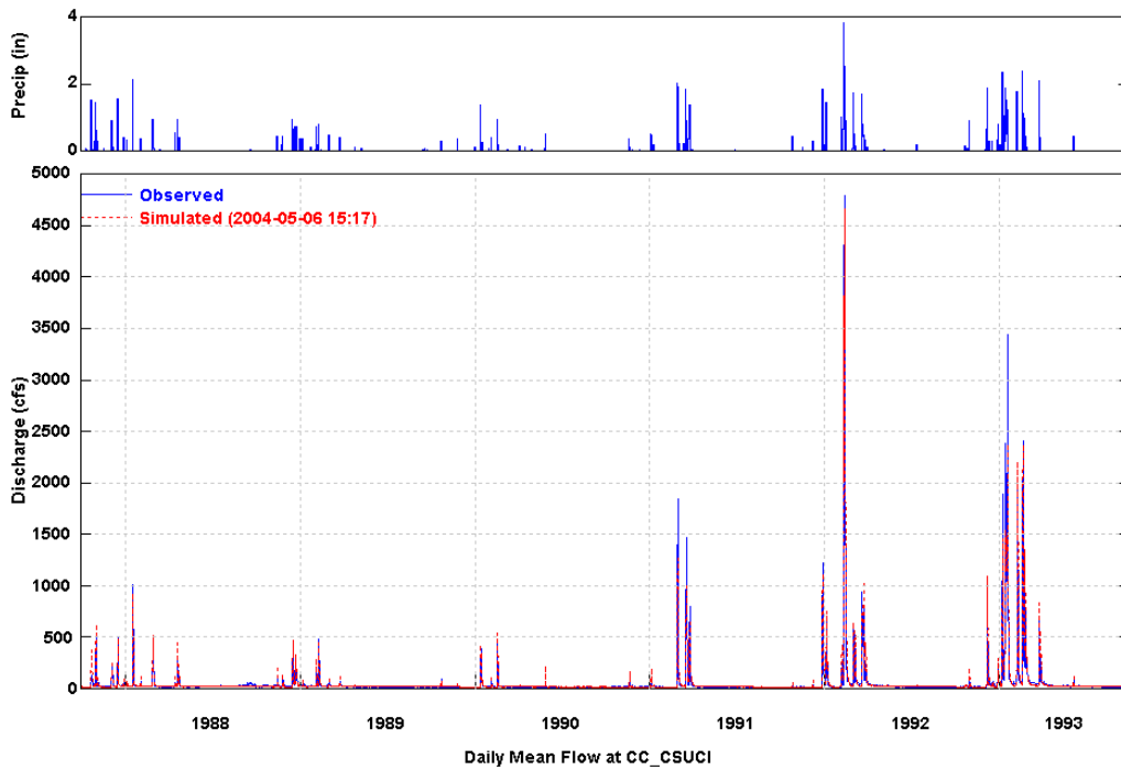
Figure 24 Simulated and Observed Daily Flow at CSUCI (WY 1988-1993)
