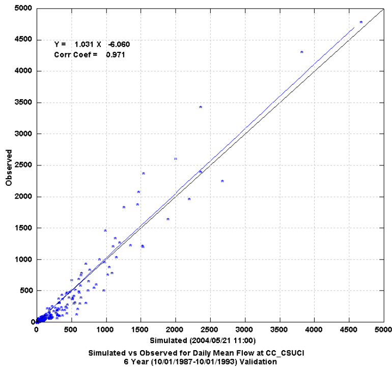
Figure 22 Daily Scatter Plot of Simulated versus Observed Flow at CSUCI
