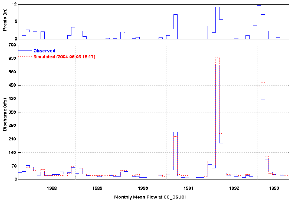
Figure 25 Simulated and Observed Monthly Flow at CSUCI (WY 1988-1993)
