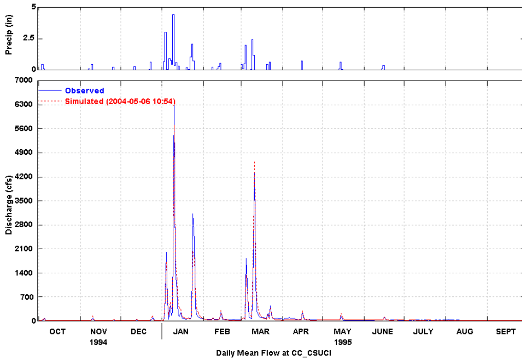
Figure 7 Simulated and Observed Daily Flow at CSUCI (WY 1995)
