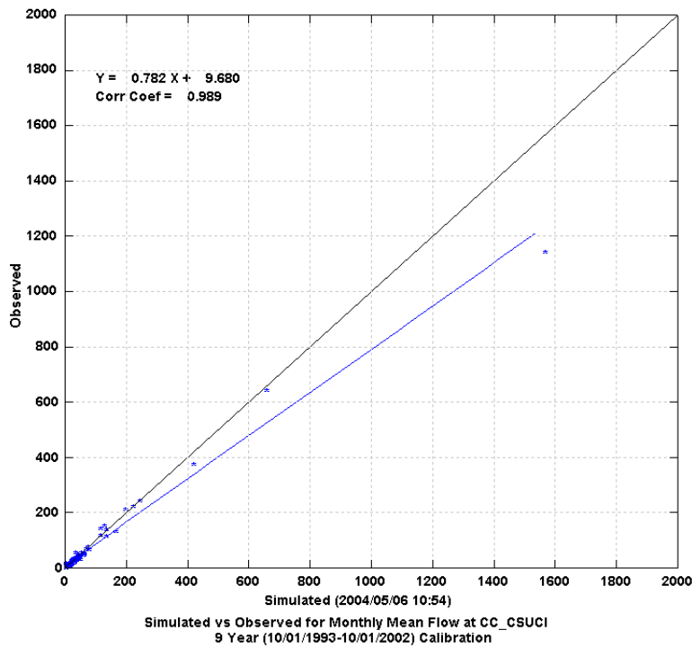
Figure 3 Monthly Scatter Plot of Simulated versus Observed Flow at CSUCI
