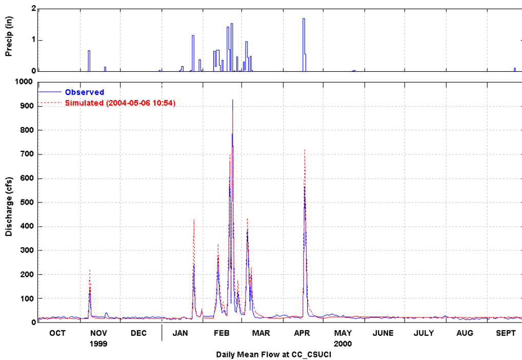
Figure 12 Simulated and Observed Daily Flow at CSUCI (WY 2000)
