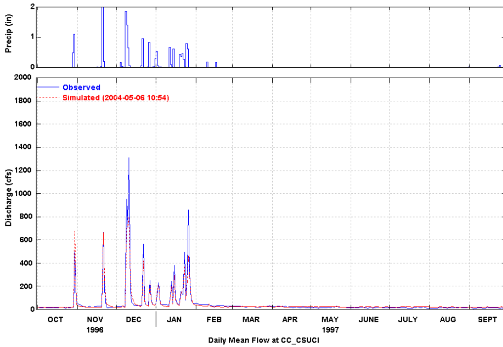
Figure 9 Simulated and Observed Daily Flow at CSUCI (WY 1997)
