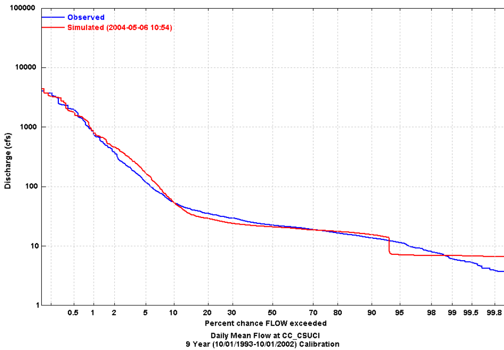
Figure 1 Simulated and Observed Daily Flow Duration Curve at CSUCI
