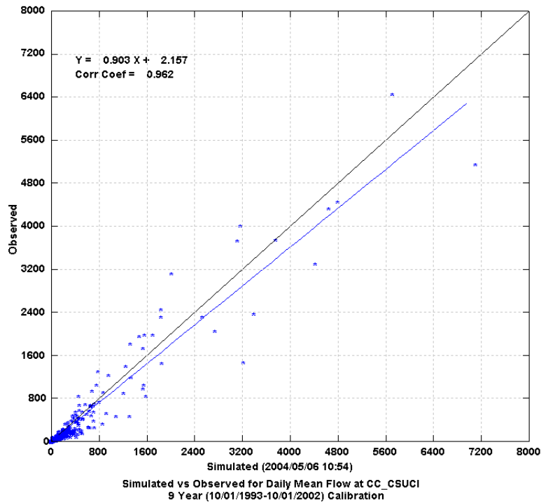
Figure 2 Daily Scatter Plot of Simulated versus Observed Flow at CSUCI
