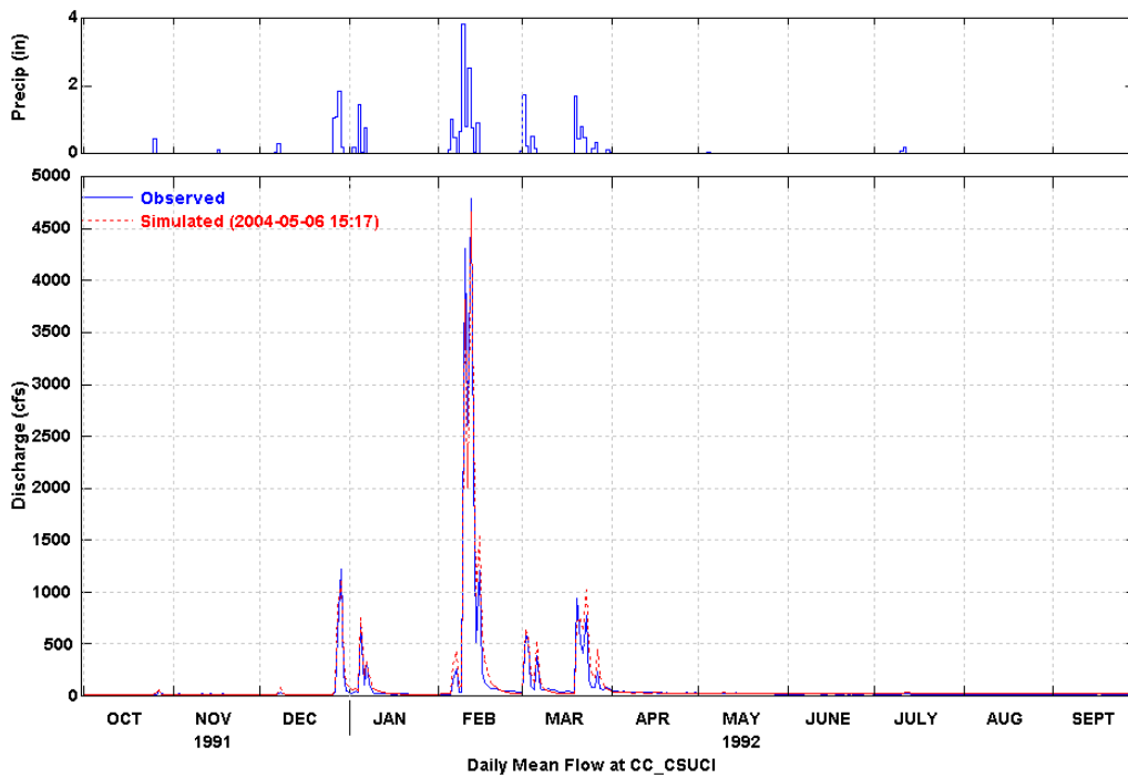
Figure 30 Simulated and Observed Daily Flow at CSUCI (WY 1992)
