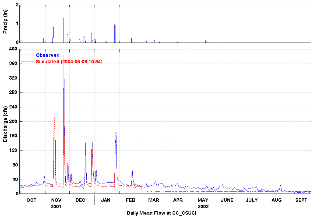
Figure 14 Simulated and Observed Daily Flow at CSUCI (WY 2002)
