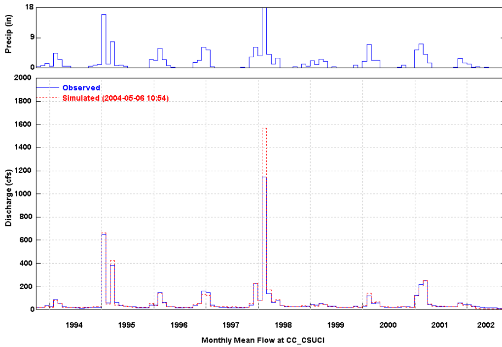
Figure 5 Simulated and Observed Monthly Flow at CSUCI (WY 1994-2002)
