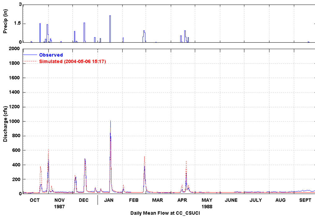
Figure 26 Simulated and Observed Daily Flow at CSUCI (WY 1988)
