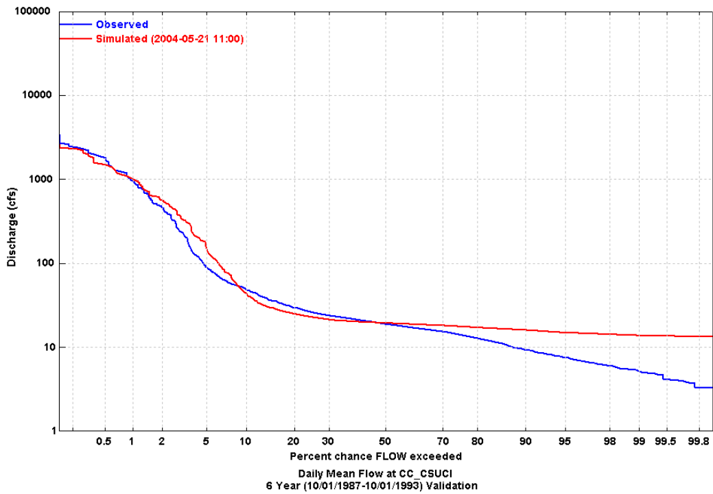
Figure 21 Simulated and Observed Daily Flow Duration Curve at CSUCI
