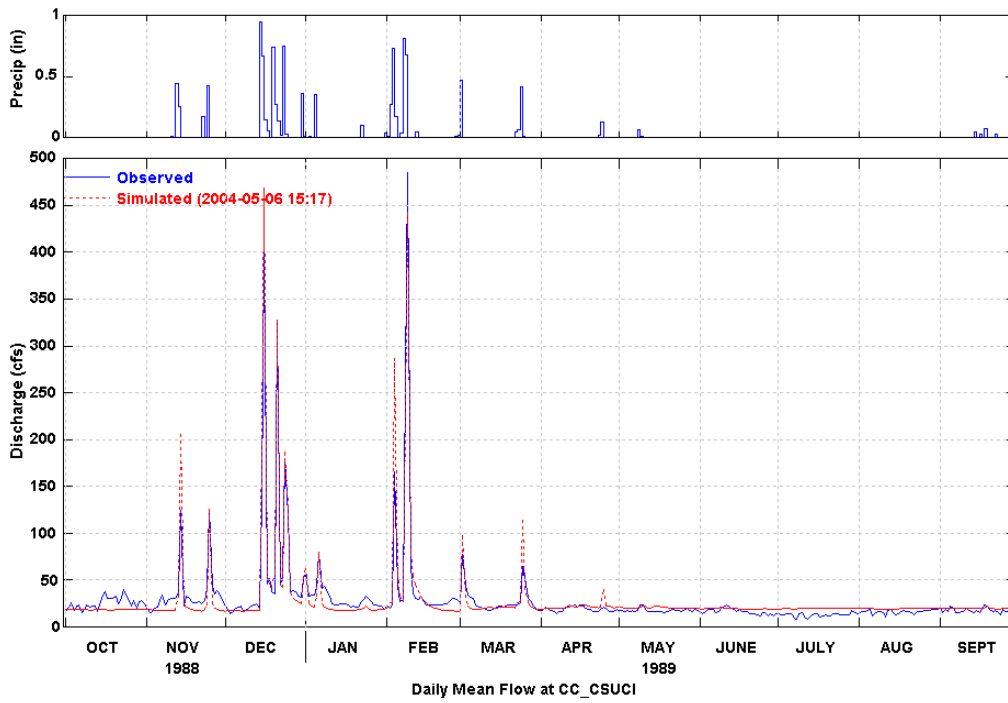
Figure 27 Simulated and Observed Daily Flow at CSUCI (WY 1989)
