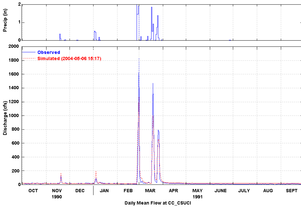
Figure 29 Simulated and Observed Daily Flow at CSUCI (WY 1991)
