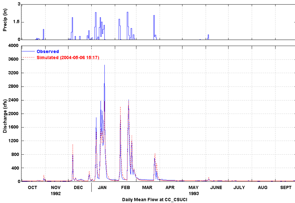
Figure 31 Simulated and Observed Daily Flow at CSUCI (WY 1993)
