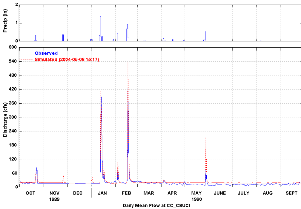
Figure 28 Simulated and Observed Daily Flow at CSUCI (WY 1990)
