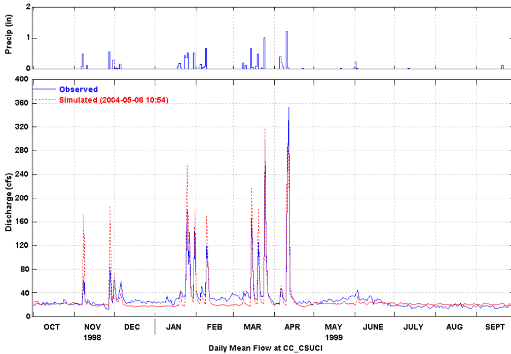
Figure 11 Simulated and Observed Daily Flow at CSUCI (WY 1999)
