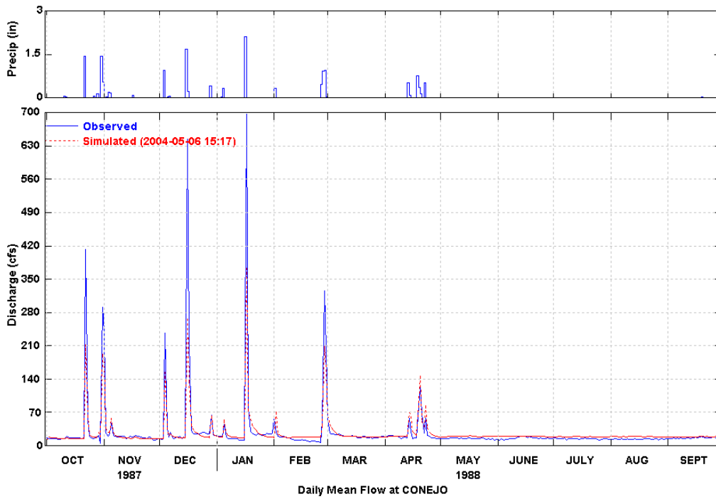
Figure 26 Simulated and Observed Daily Flow at Conejo (WY 1988)
