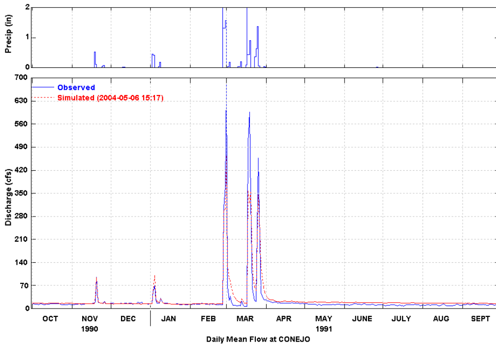
Figure 29 Simulated and Observed Daily Flow at Conejo (WY 1991)
