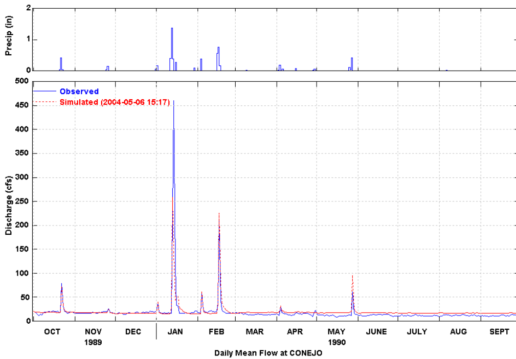
Figure 28 Simulated and Observed Daily Flow at Conejo (WY 1990)
