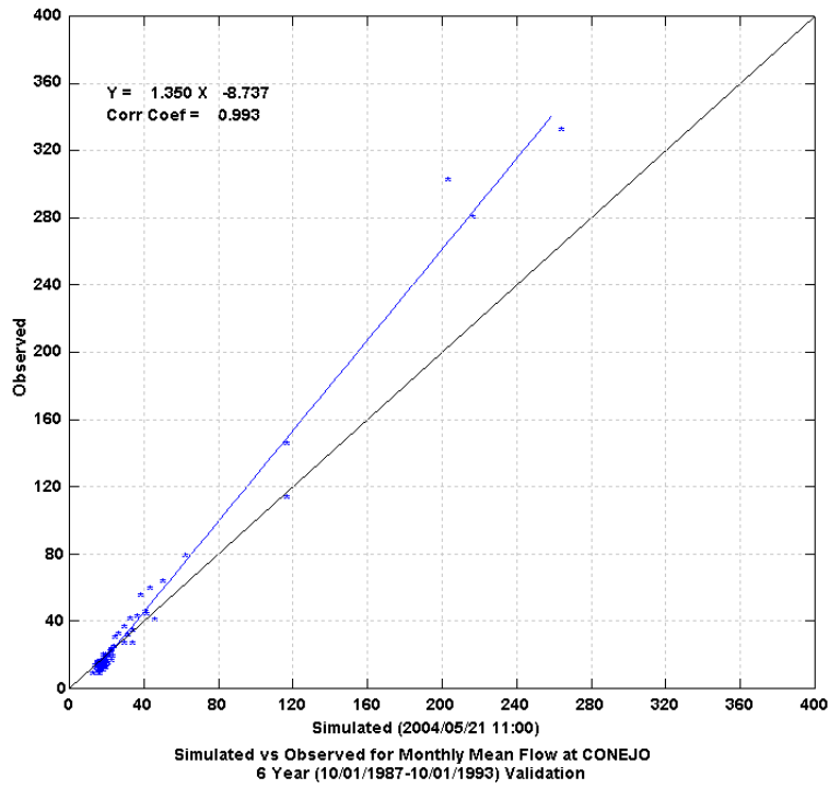
Figure 23 Monthly Scatter Plot of Simulated versus Observed Flow at Conejo
