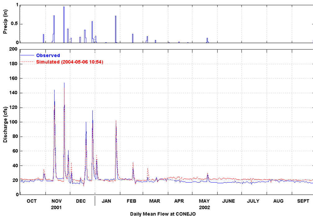
Figure 14 Simulated and Observed Daily Flow at Conejo (WY 2002)
