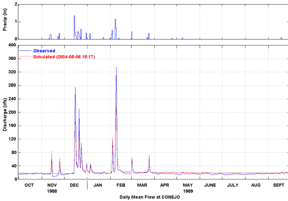
Figure 27 Simulated and Observed Daily Flow at Conejo (WY 1989)
