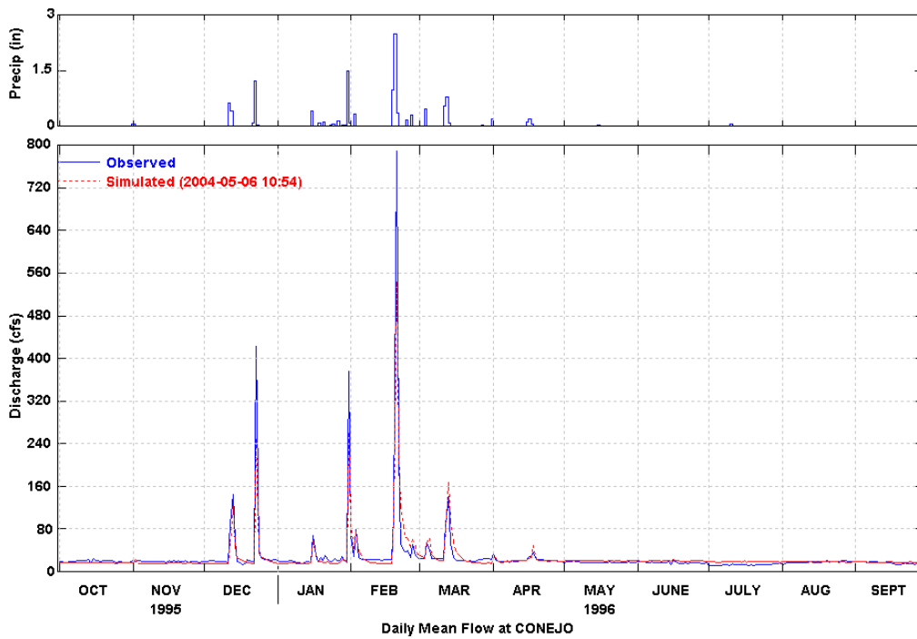
Figure 8 Simulated and Observed Daily Flow at Conejo (WY 1996)
