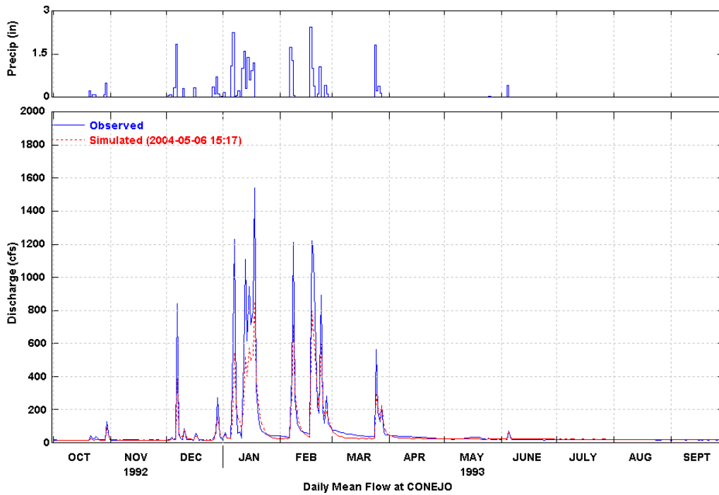
Figure 31 Simulated and Observed Daily Flow at Conejo (WY 1993)
