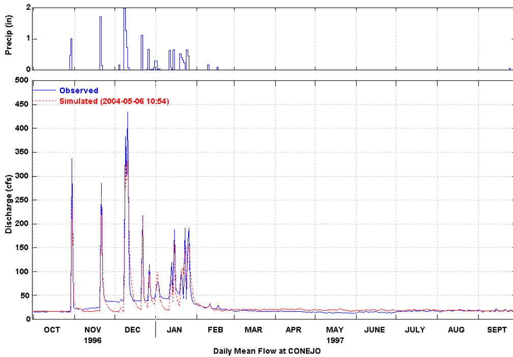
Figure 9 Simulated and Observed Daily Flow at Conejo (WY 1997)
