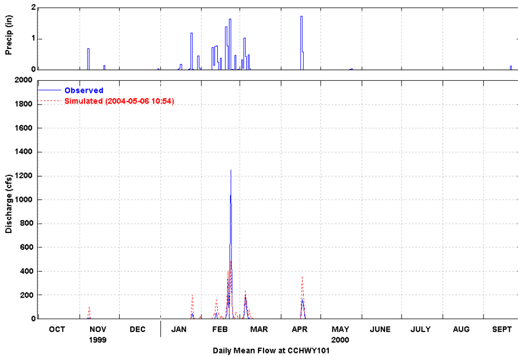
Figure 12 Simulated and Observed Daily Flow at Conejo (WY 2000)
