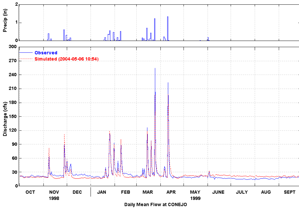
Figure 11 Simulated and Observed Daily Flow at Conejo (WY 1999)
