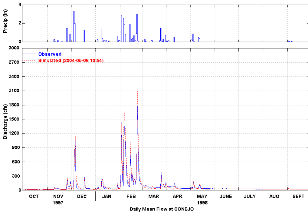
Figure 10 Simulated and Observed Daily Flow at Conejo (WY 1998)
