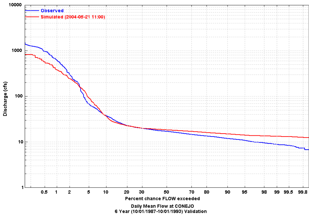
Figure 21 Simulated and Observed Daily Flow Duration Curve at Conejo
