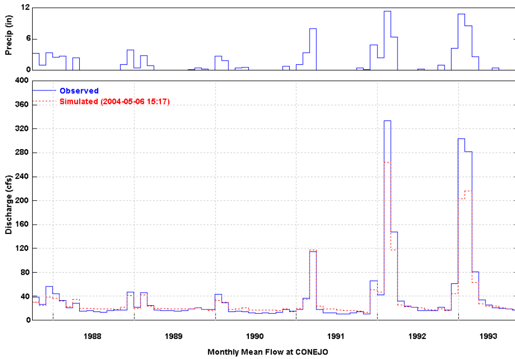
Figure 25 Simulated and Observed Monthly Flow at Conejo (WY 1988-1993)
