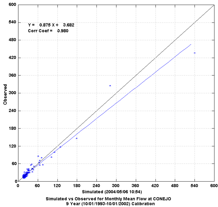
Figure 3 Monthly Scatter Plot of Simulated versus Observed Flow at Conejo
