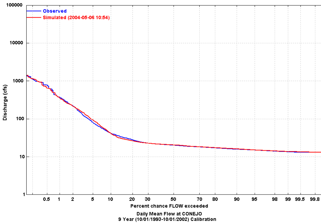
Figure 1 Simulated and Observed Daily Flow Duration Curve at Conejo
