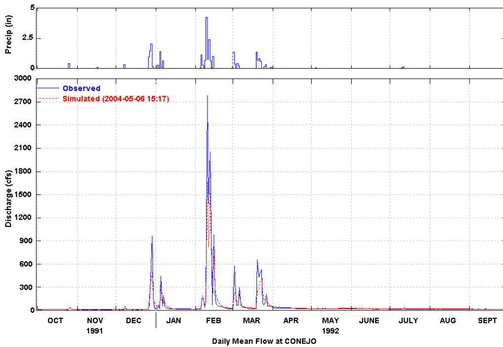
Figure 30 Simulated and Observed Daily Flow at Conejo (WY 1992)
