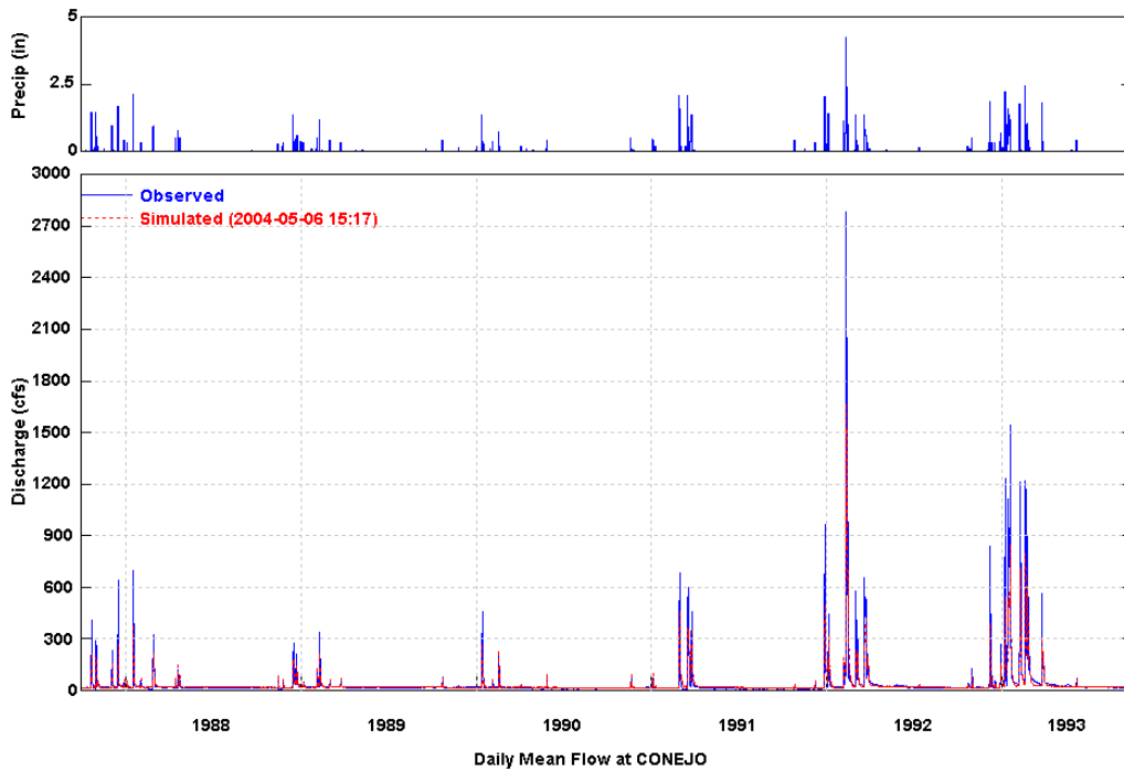
Figure 24 Simulated and Observed Daily Flow at Conejo (WY 1988-1993)
