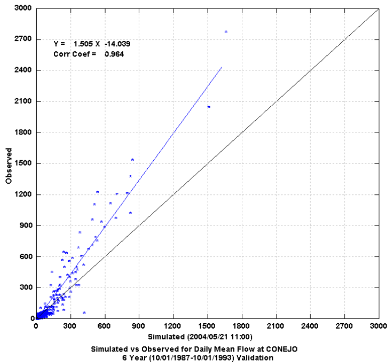
Figure 22 Daily Scatter Plot of Simulated versus Observed Flow at Conejo
