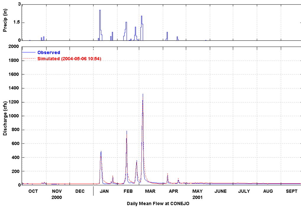
Figure 13 Simulated and Observed Daily Flow at Conejo (WY 2001)
