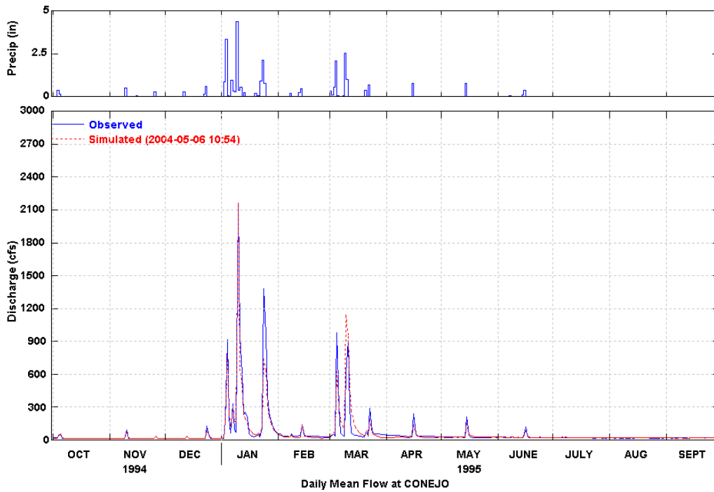
Figure 7 Simulated and Observed Daily Flow at Conejo (WY 1995)
