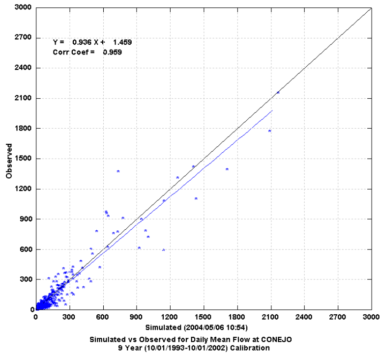
Figure 2 Daily Scatter Plot of Simulated versus Observed Flow at Conejo
