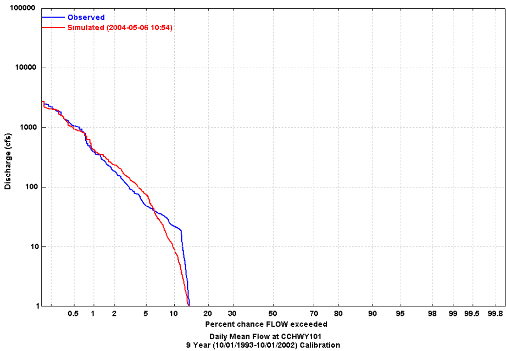
Figure 1 Simulated and Observed Daily Flow Duration Curve at Hyw. 101
