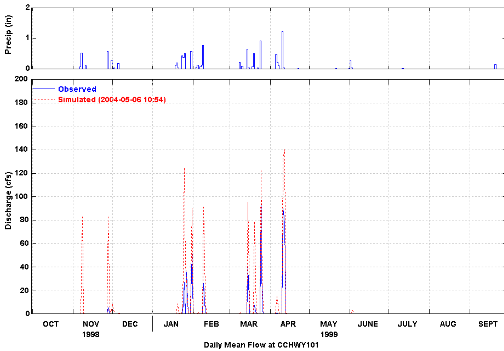
Figure 11 Simulated and Observed Daily Flow at Hyw. 101 (WY 1999)
