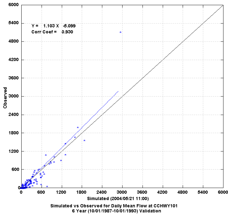
Figure 22 Daily Scatter Plot of Simulated versus Observed Flow at Hyw. 101
