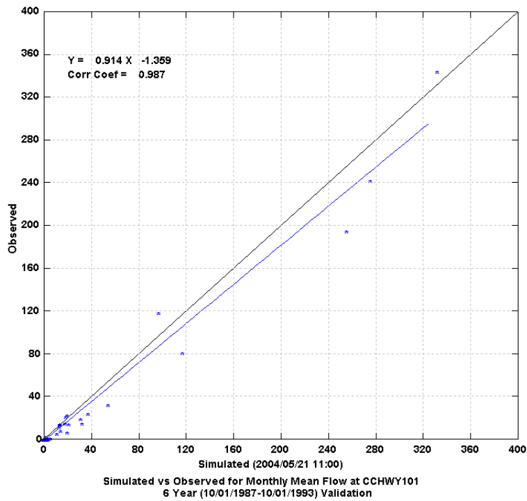
Figure 23 Monthly Scatter Plot of Simulated versus Observed Flow at Hyw. 101
