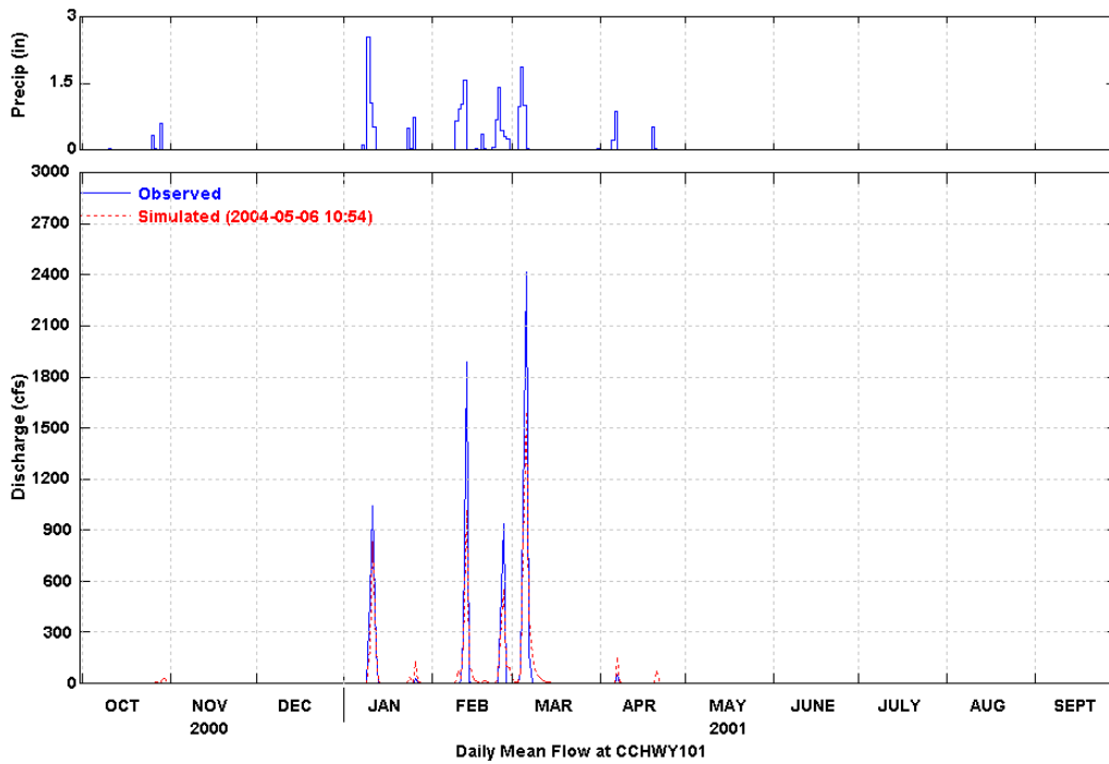
Figure 13 Simulated and Observed Daily Flow at Hyw. 101 (WY 2001)
