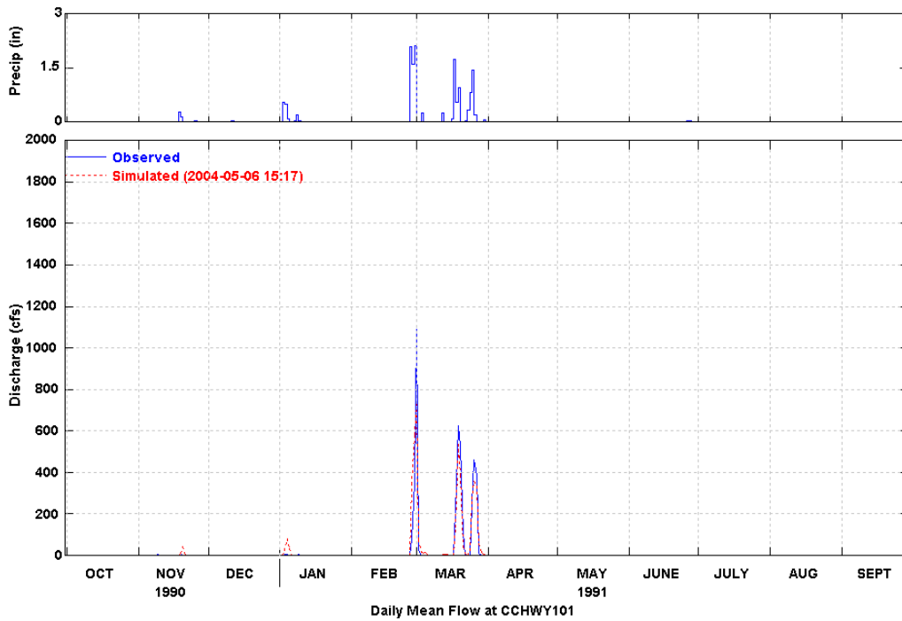
Figure 29 Simulated and Observed Daily Flow at Hyw. 101 (WY 1991)
