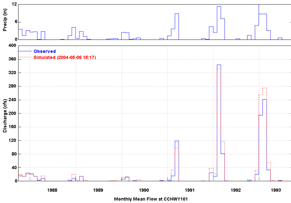
Figure 25 Simulated and Observed Monthly Flow at Hyw. 101 (WY 1988-1993)
