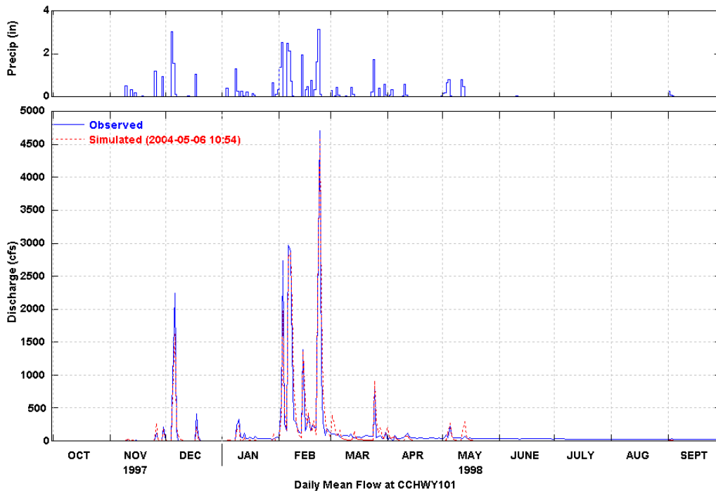
Figure 9 Simulated and Observed Daily Flow at Hyw. 101 (WY 1997)
