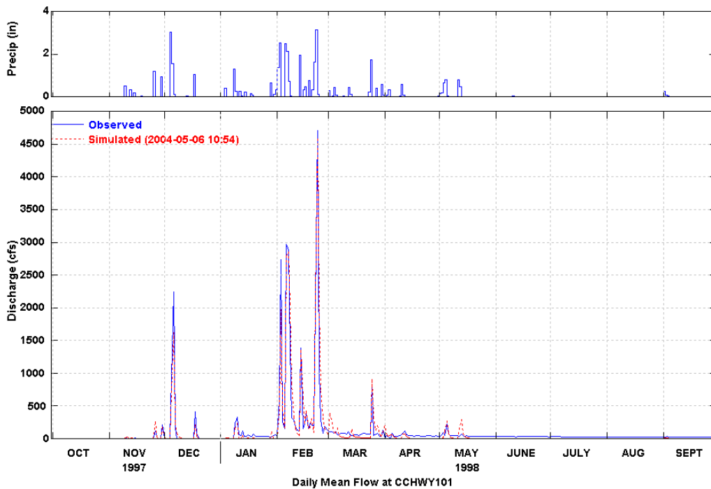
Figure 10 Simulated and Observed Daily Flow at Hyw. 101 (WY 1998)
