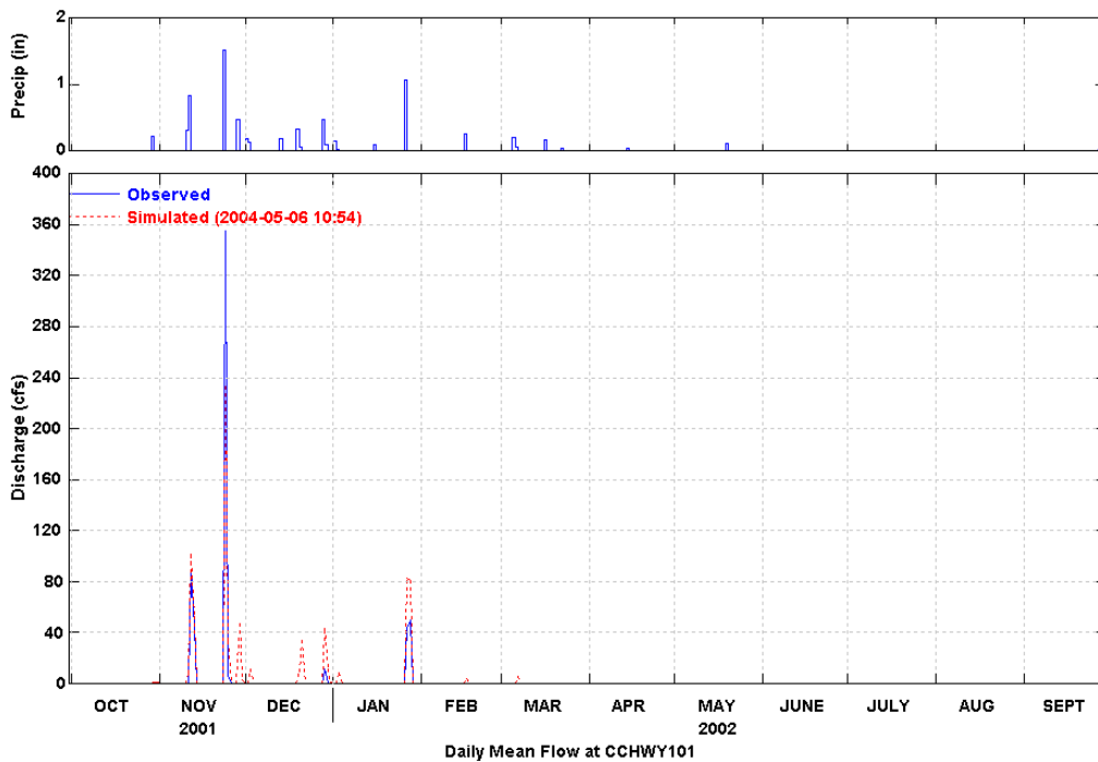
Figure 14 Simulated and Observed Daily Flow at Hyw. 101 (WY 2002)
