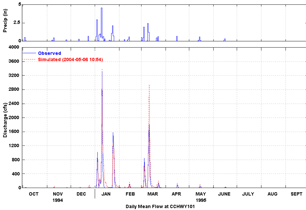
Figure 7 Simulated and Observed Daily Flow at Hyw. 101 (WY 1995)
