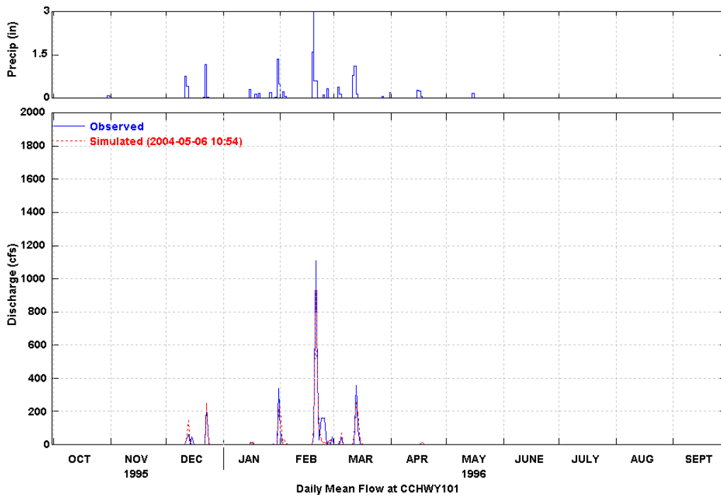
Figure 8 Simulated and Observed Daily Flow at Hyw. 101 (WY 1996)
