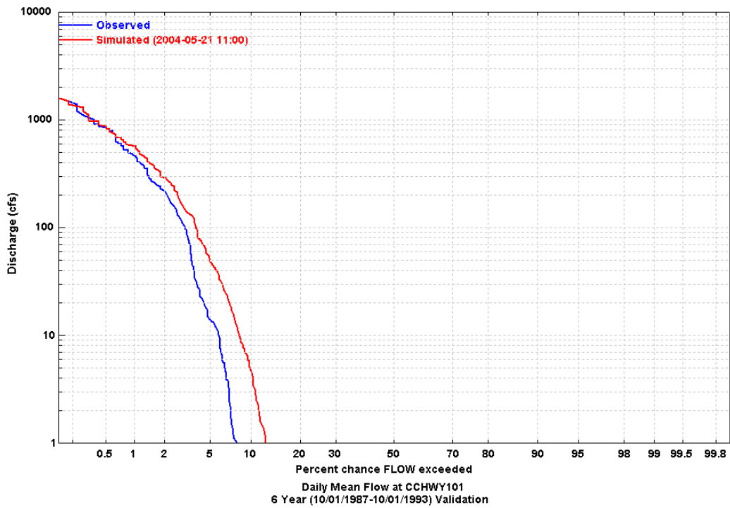
Figure 21 Simulated and Observed Daily Flow Duration Curve at Hyw. 101
