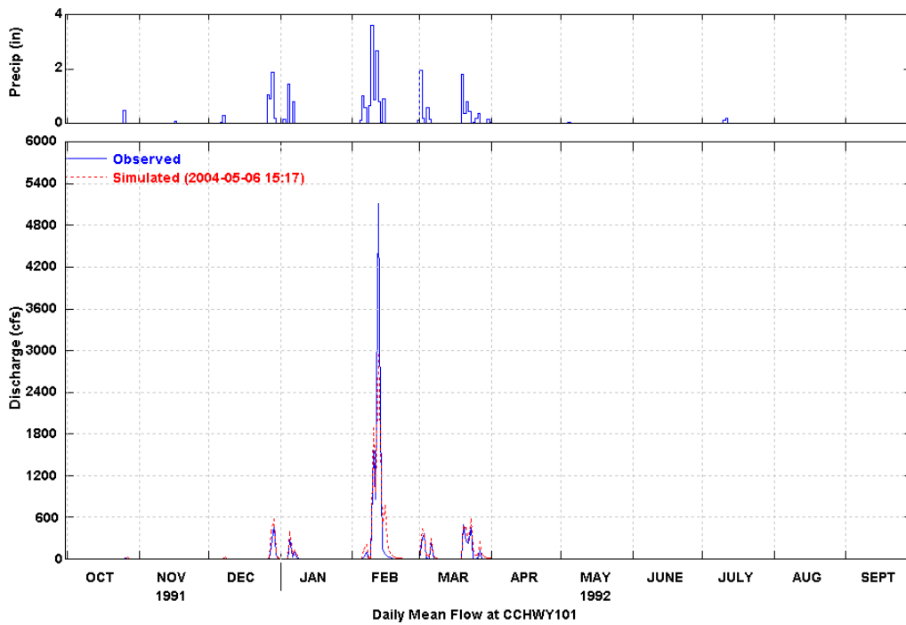
Figure 30 Simulated and Observed Daily Flow at Hyw. 101 (WY 1992)
