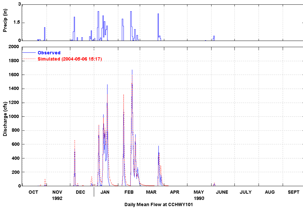
Figure 31 Simulated and Observed Daily Flow at Hyw. 101 (WY 1993)
