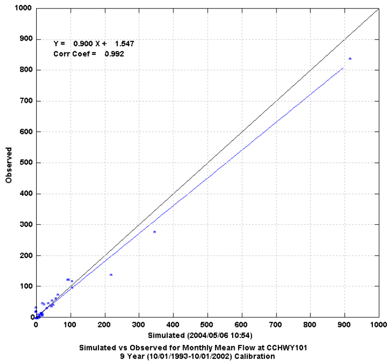
Figure 3 Monthly Scatter Plot of Simulated versus Observed Flow at Hyw. 101
