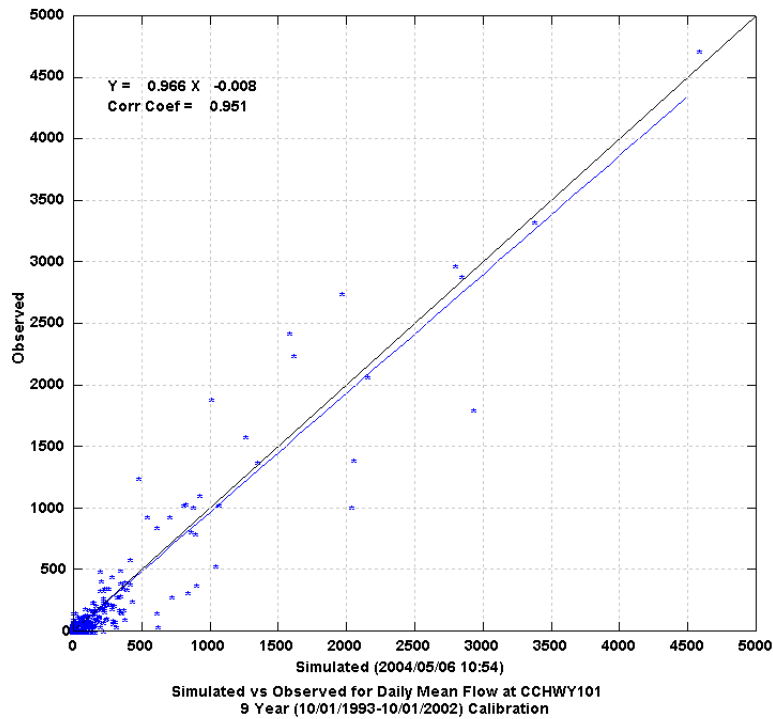
Figure 2 Daily Scatter Plot of Simulated versus Observed Flow at Hyw. 101
