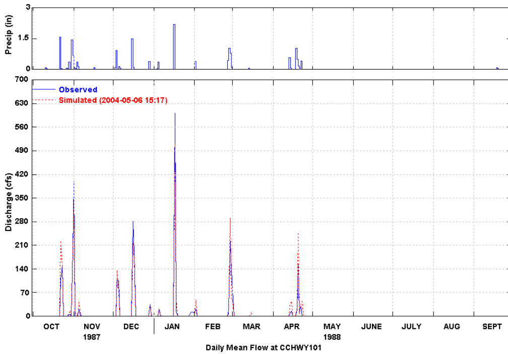
Figure 26 Simulated and Observed Daily Flow at Hyw. 101 (WY 1988)
