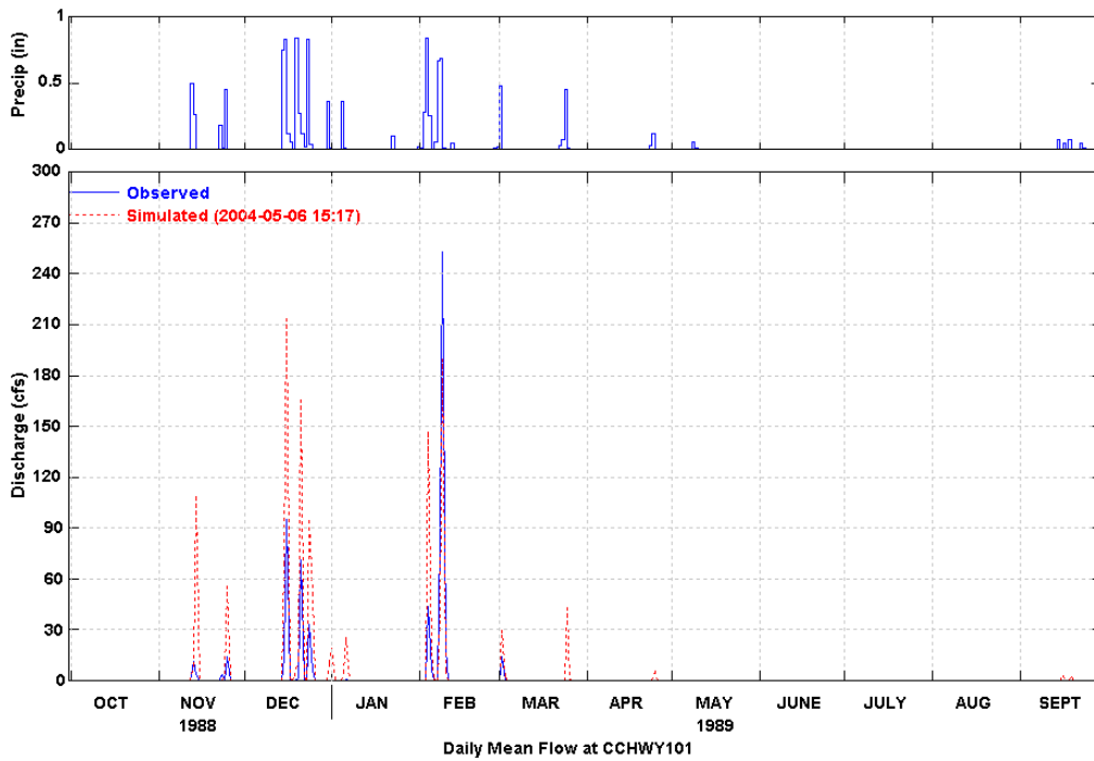
Figure 27 Simulated and Observed Daily Flow at Hyw. 101 (WY 1989)
