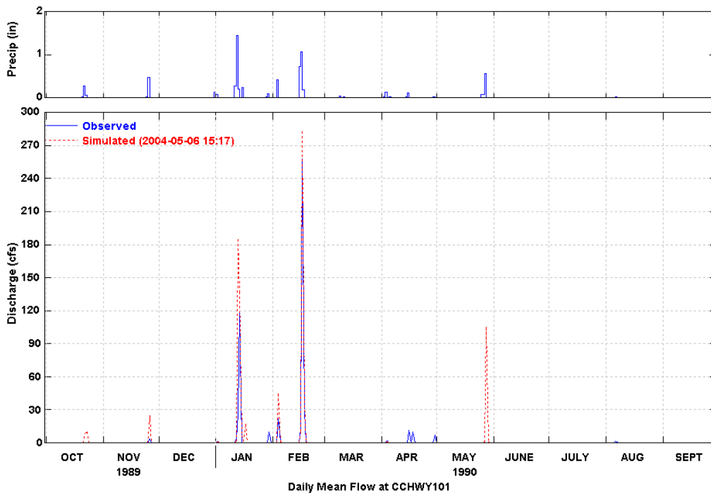
Figure 28 Simulated and Observed Daily Flow at Hyw. 101 (WY 1990)
