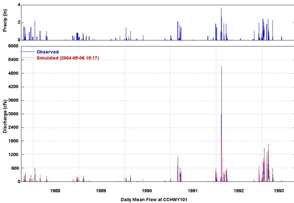
Figure 24 Simulated and Observed Daily Flow at Hyw. 101 (WY 1988-1993)
