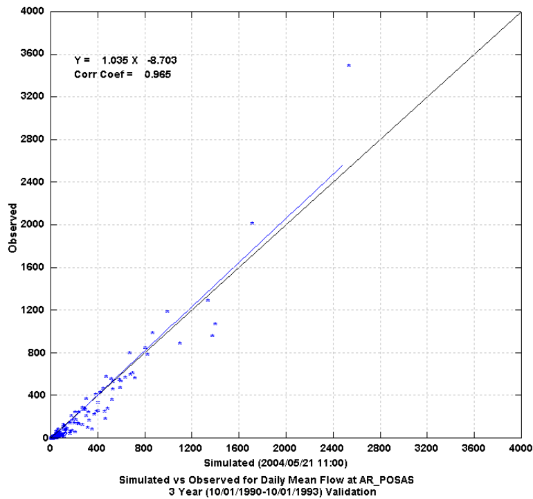
Figure 22 Daily Scatter Plot of Simulated versus Observed Flow at Hitch Blvd.
