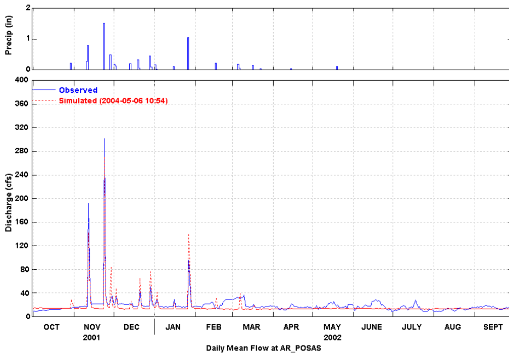
Figure 14 Simulated and Observed Daily Flow at Hitch Blvd. (WY 2002)
