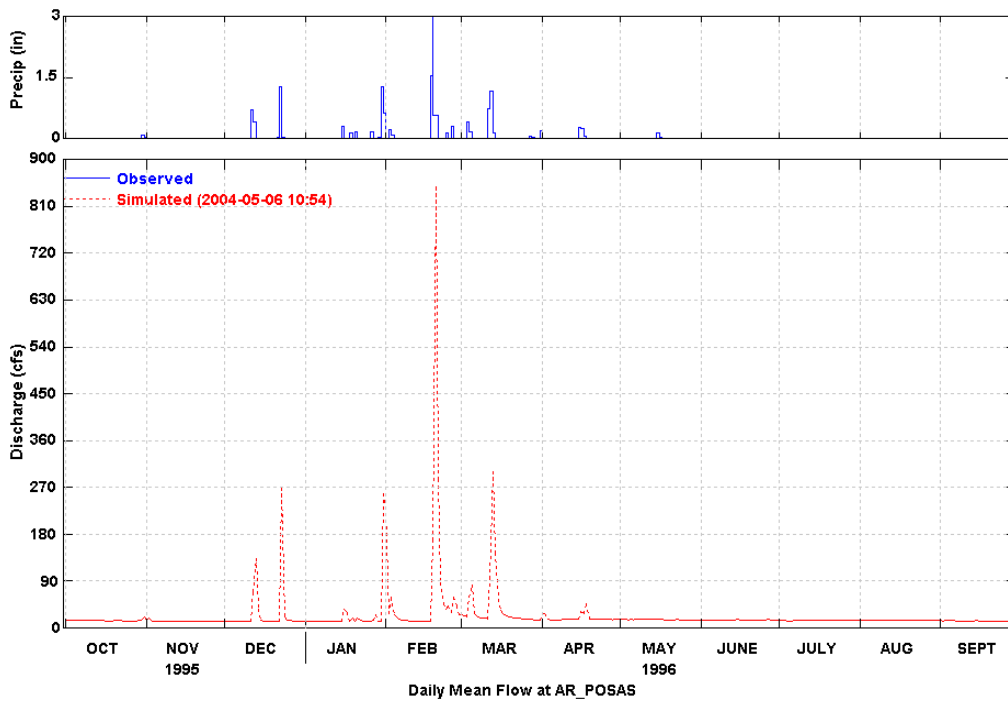
Figure 8 Simulated and Observed Daily Flow at Hitch Blvd. (WY 1996)
