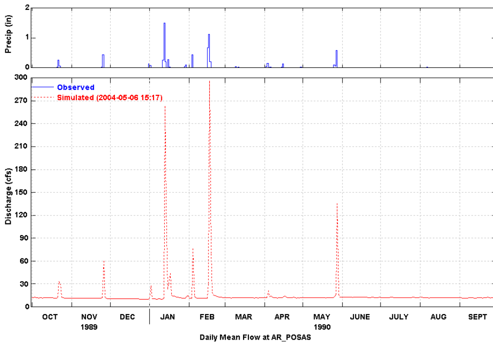
Figure 28 Simulated and Observed Daily Flow at Hitch Blvd. (WY 1990)
