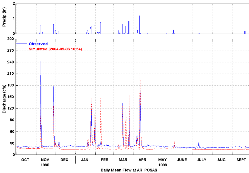
Figure 11 Simulated and Observed Daily Flow at Hitch Blvd. (WY 1999)
