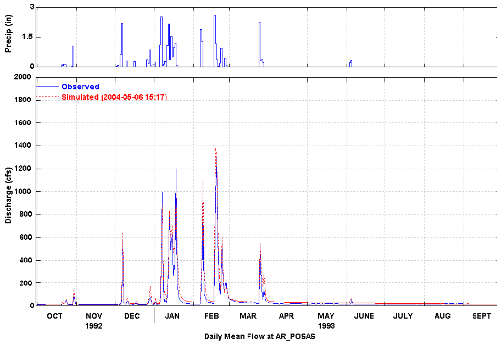
Figure 31 Simulated and Observed Daily Flow at Hitch Blvd. (WY 1993)
