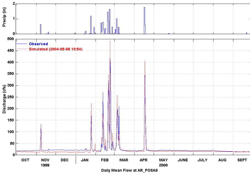
Figure 12 Simulated and Observed Daily Flow at Hitch Blvd. (WY 2000)
