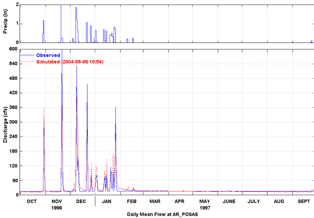
Figure 9 Simulated and Observed Daily Flow at Hitch Blvd. (WY 1997)
