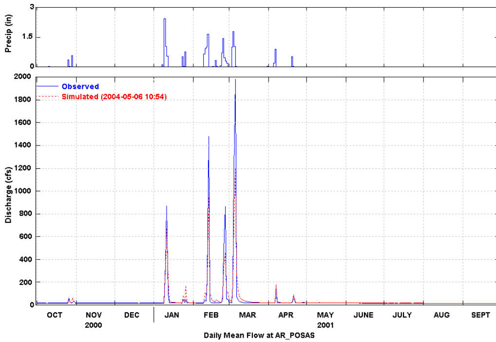
Figure 13 Simulated and Observed Daily Flow at Hitch Blvd. (WY 2001)
