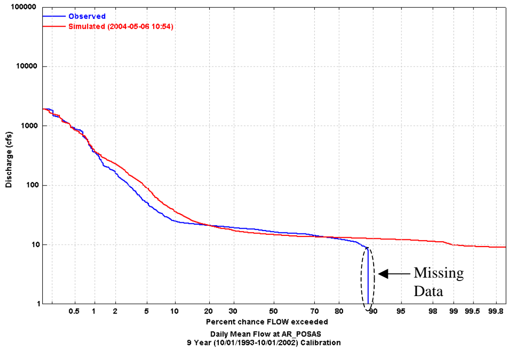
Figure 1 Simulated and Observed Daily Flow Duration Curve at Hitch Blvd.
