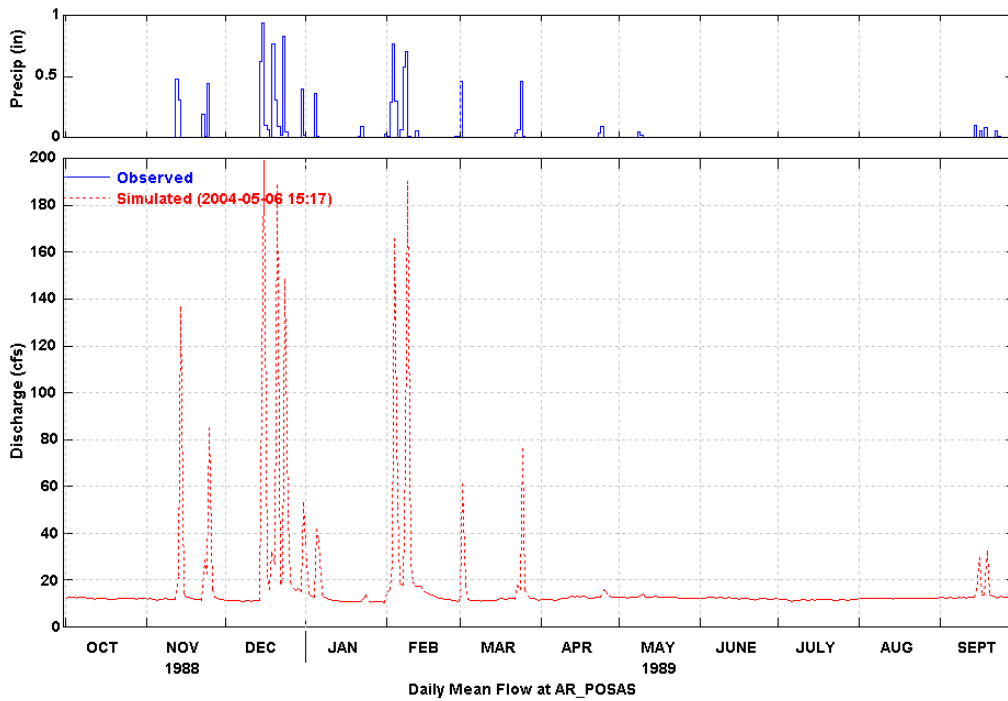
Figure 27 Simulated and Observed Daily Flow at Hitch Blvd. (WY 1989)
