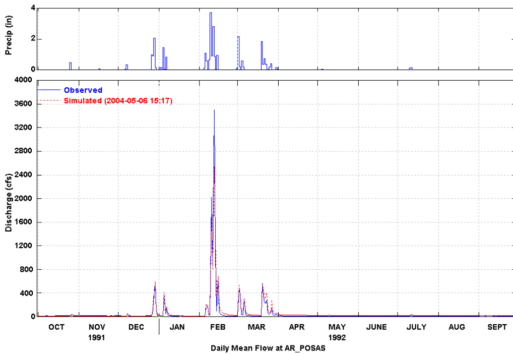
Figure 30 Simulated and Observed Daily Flow at Hitch Blvd. (WY 1992)
