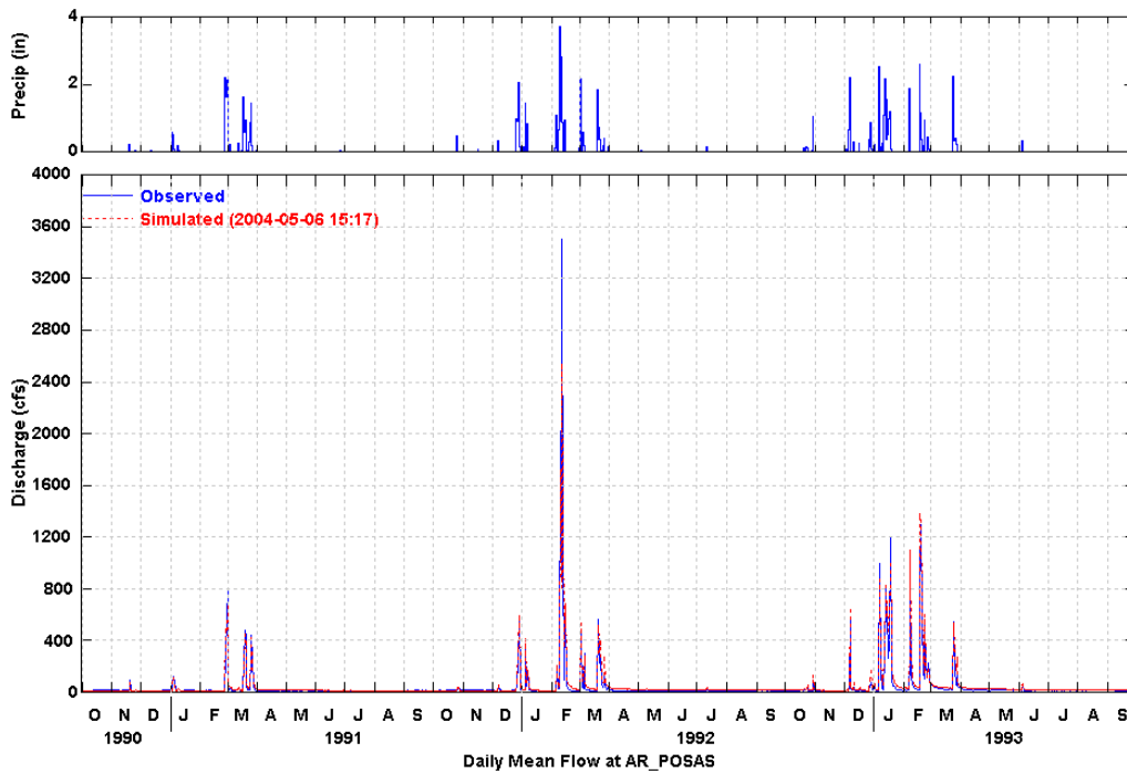
Figure 24 Simulated and Observed Daily Flow at Hitch Blvd. (WY 1988-1993)
