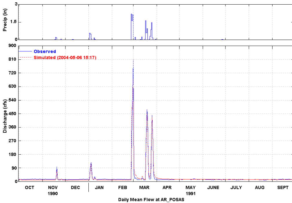
Figure 29 Simulated and Observed Daily Flow at Hitch Blvd. (WY 1991)
