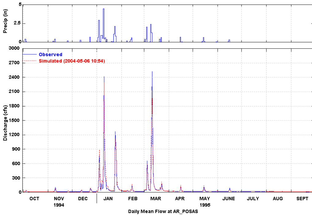
Figure 7 Simulated and Observed Daily Flow at Hitch Blvd. (WY 1995)
