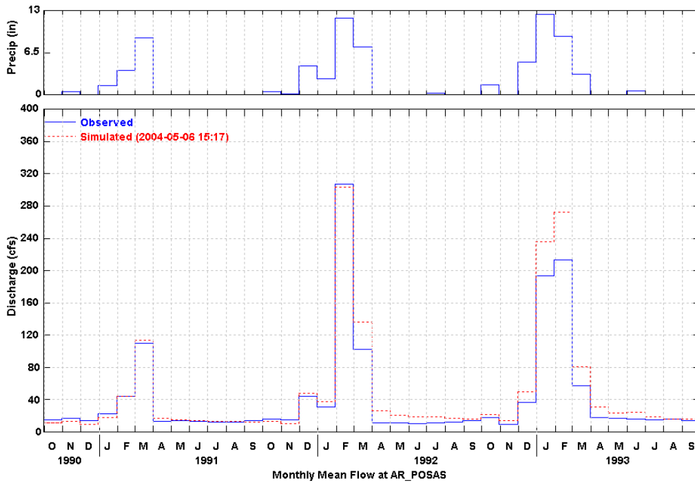
Figure 25 Simulated and Observed Monthly Flow at Hitch Blvd. (WY 1994-2002)
