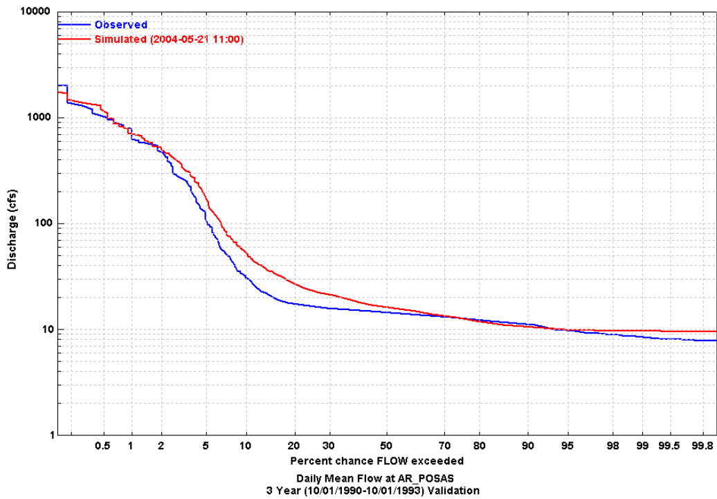
Figure 21 Simulated and Observed Daily Flow Duration Curve at Hitch Blvd.
