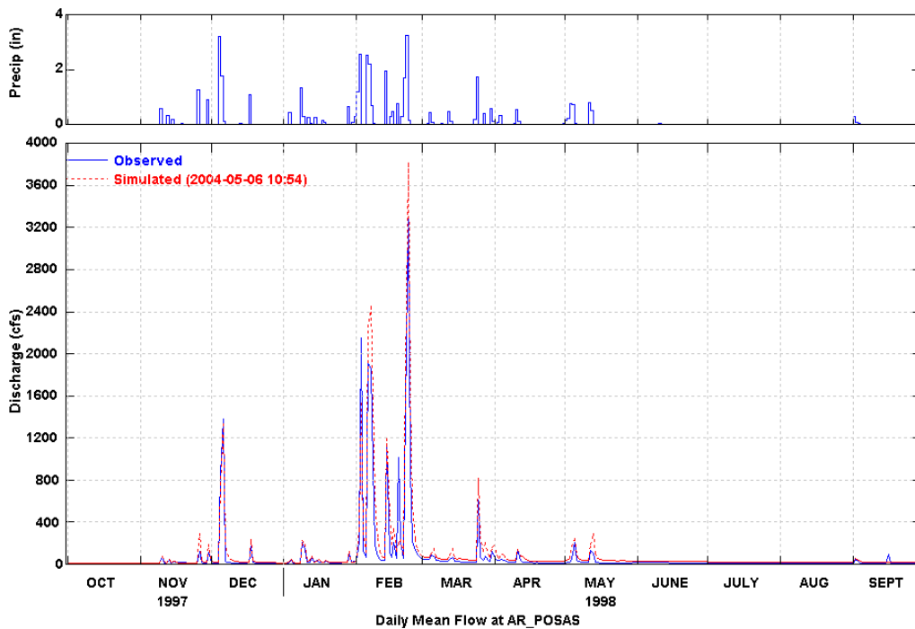
Figure 10 Simulated and Observed Daily Flow at Hitch Blvd. (WY 1998)
