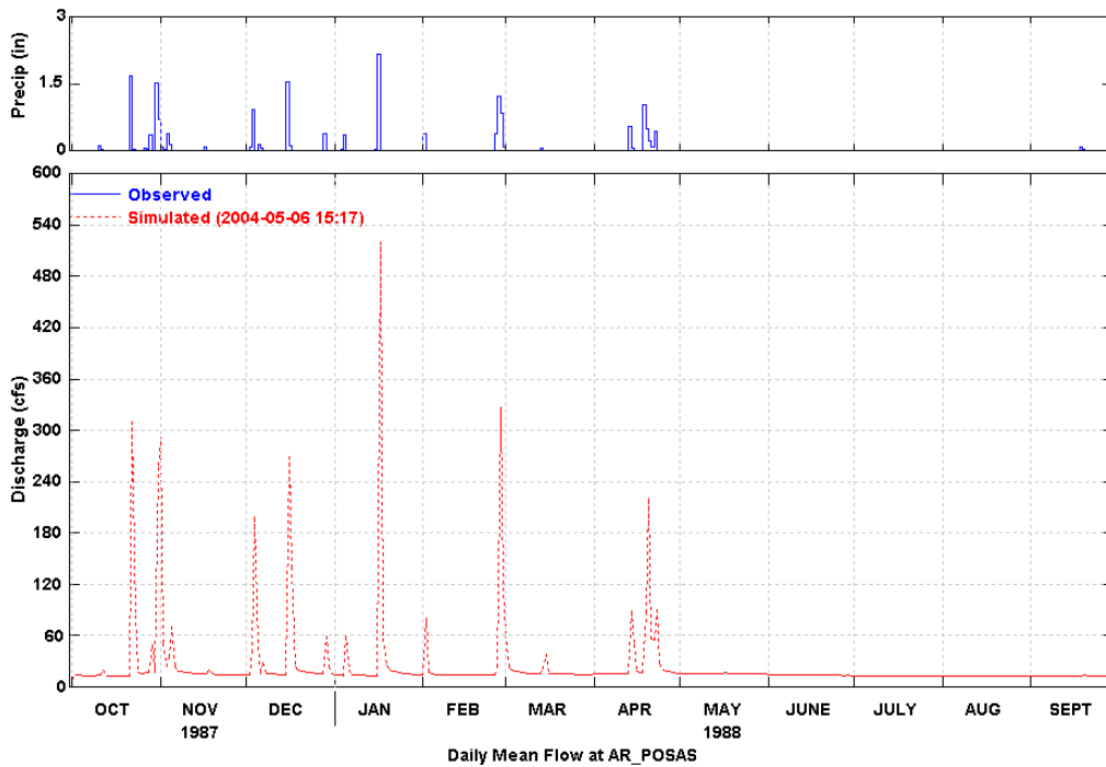
Figure 26 Simulated and Observed Daily Flow at Hitch Blvd. (WY 1988)
