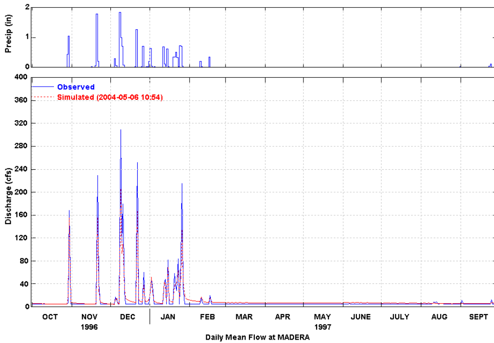
Figure 9 Simulated and Observed Daily Flow at Madera (WY 1997)
