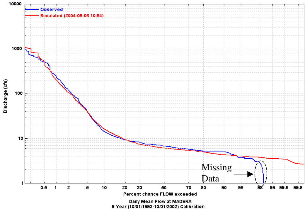
Figure 1 Simulated and Observed Daily Flow Duration Curve at Madera
