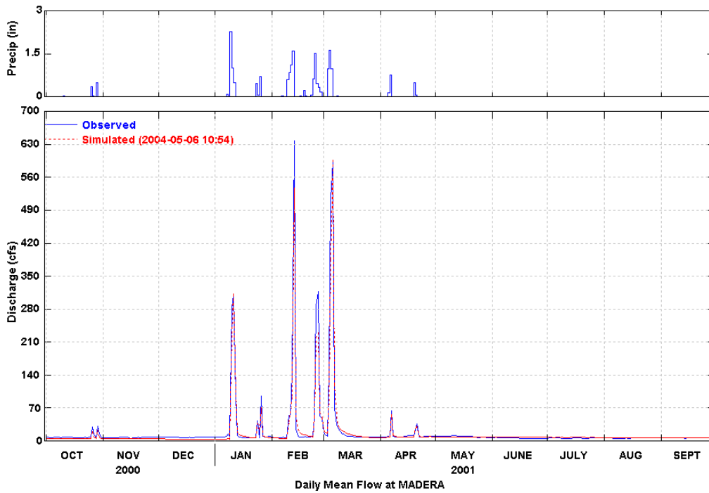
Figure 13 Simulated and Observed Daily Flow at Madera (WY 2001)
