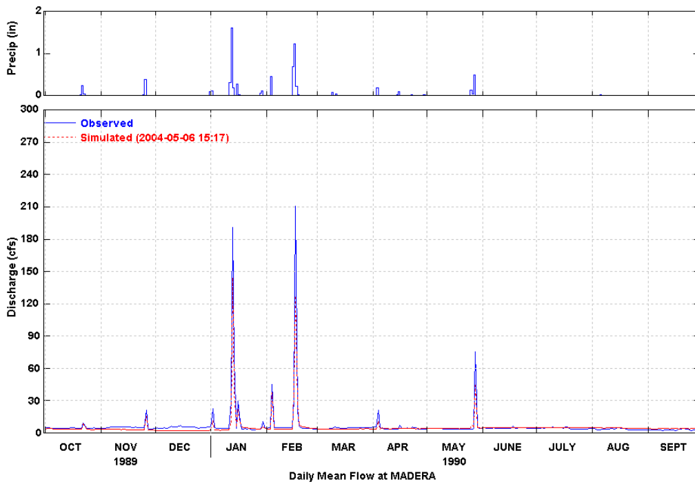
Figure 28 Simulated and Observed Daily Flow at Madera (WY 1990)
