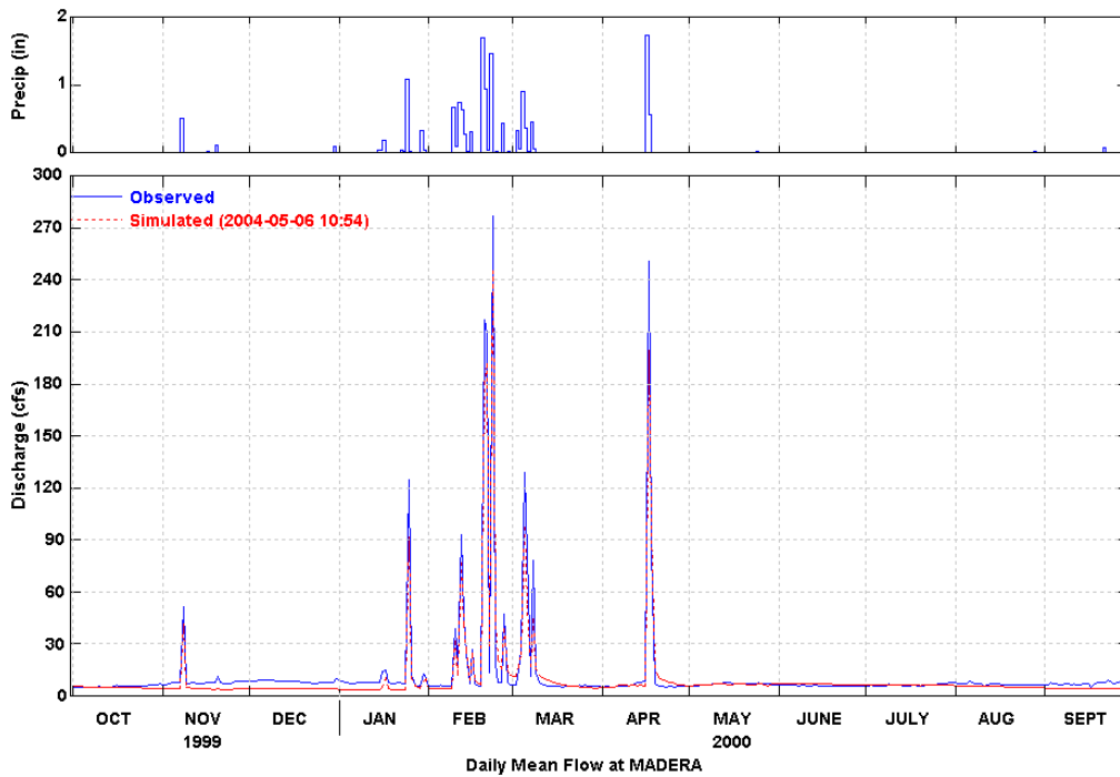
Figure 12 Simulated and Observed Daily Flow at Madera (WY 2000)
