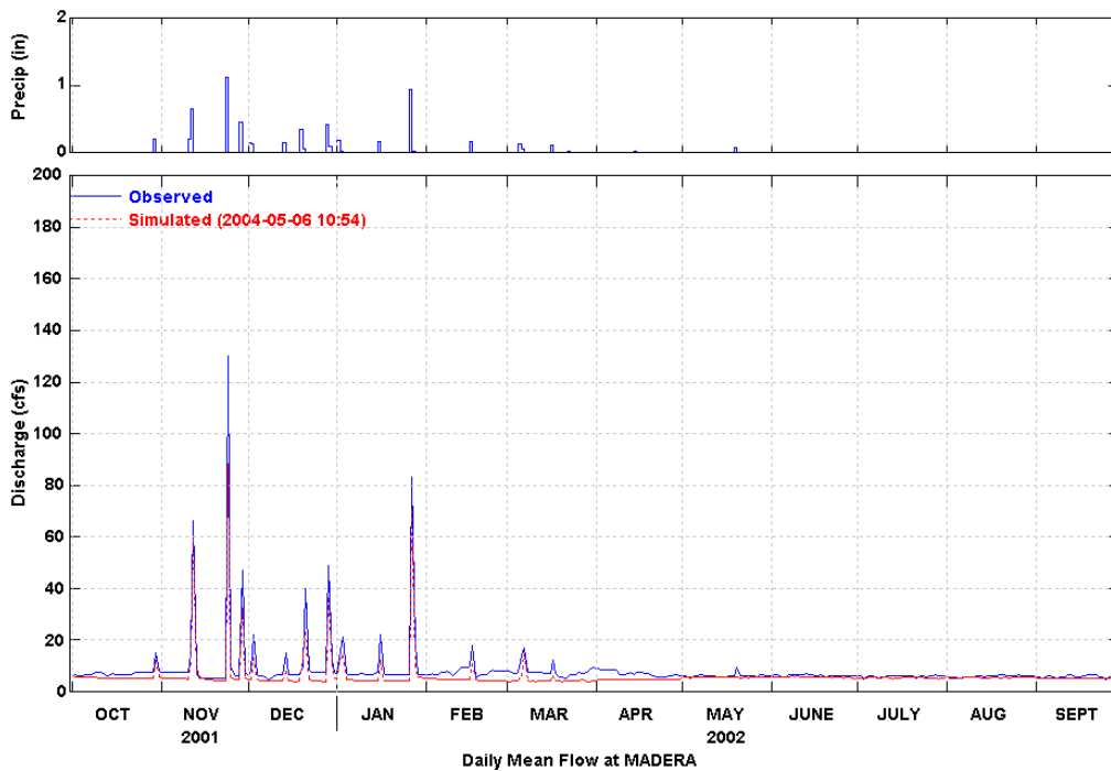
Figure 14 Simulated and Observed Daily Flow at Madera (WY 2002)
