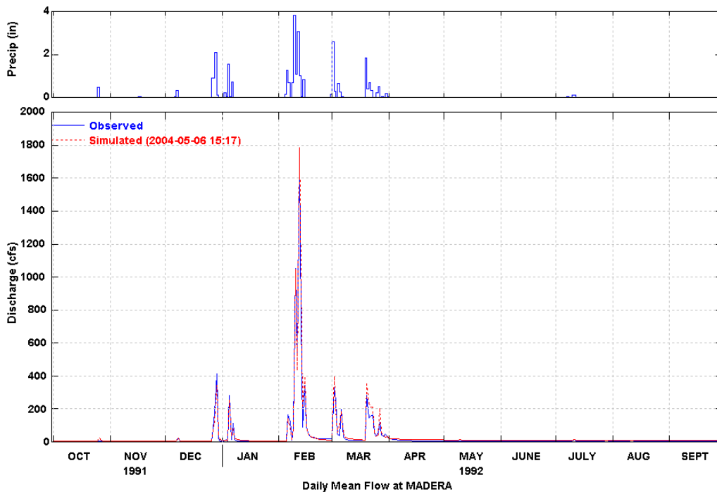
Figure 30 Simulated and Observed Daily Flow at Madera (WY 1992)
