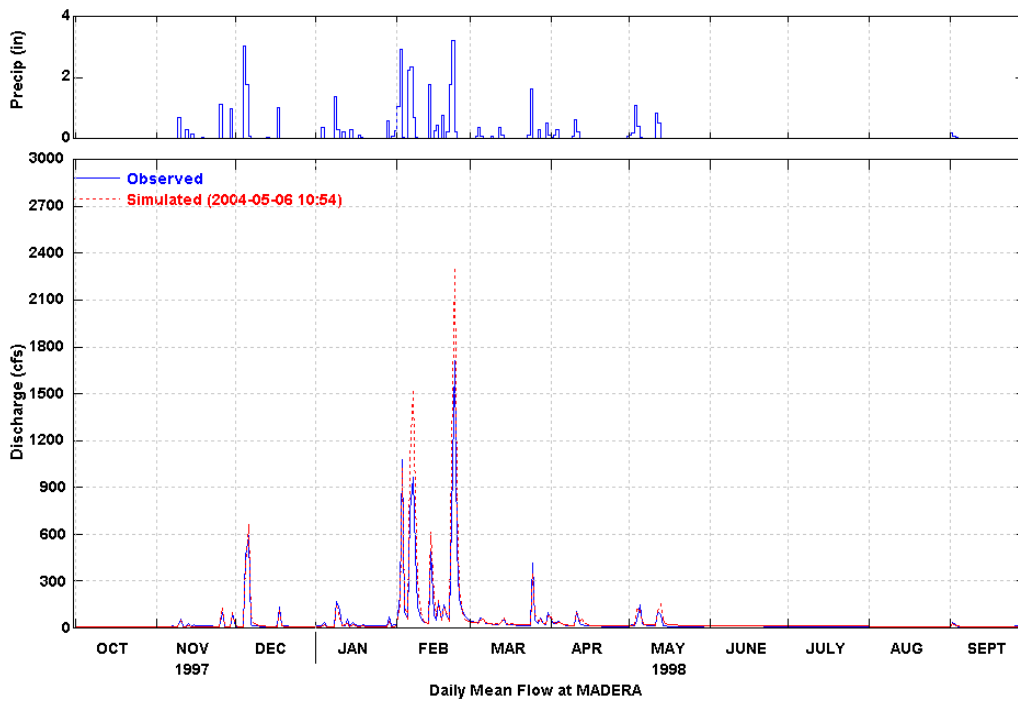
Figure 10 Simulated and Observed Daily Flow at Madera (WY 1998)
