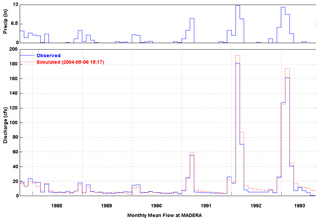
Figure 25 Simulated and Observed Monthly Flow at Madera (WY 1988-1993)
