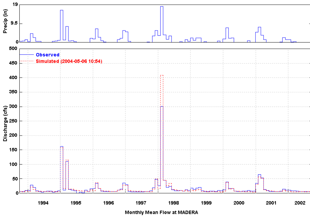
Figure 5 Simulated and Observed Monthly Flow at Madera (WY 1994-2002)
