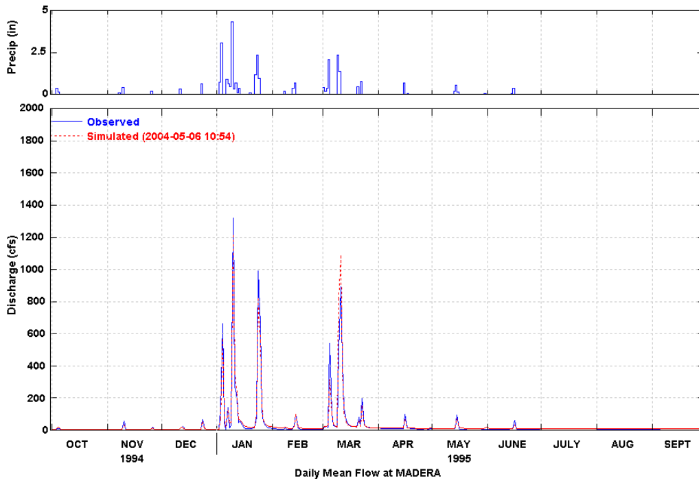
Figure 7 Simulated and Observed Daily Flow at Madera (WY 1995)
