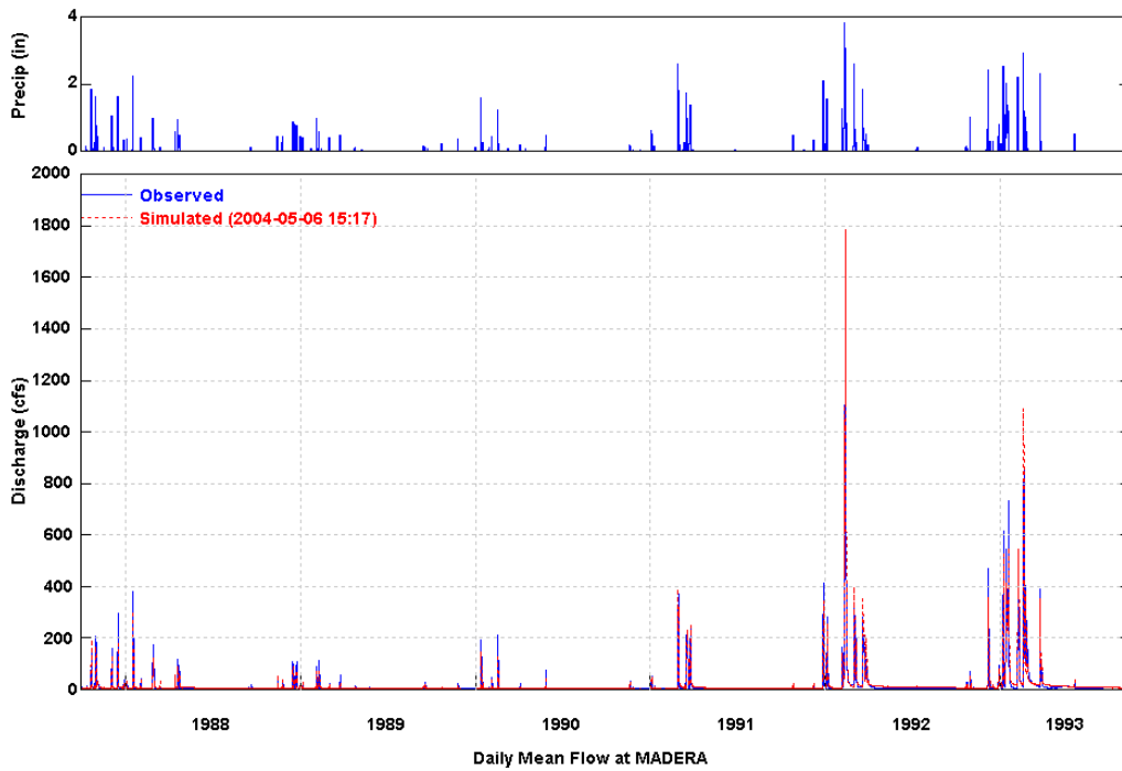
Figure 24 Simulated and Observed Daily Flow at Madera (WY 1988-1993)
