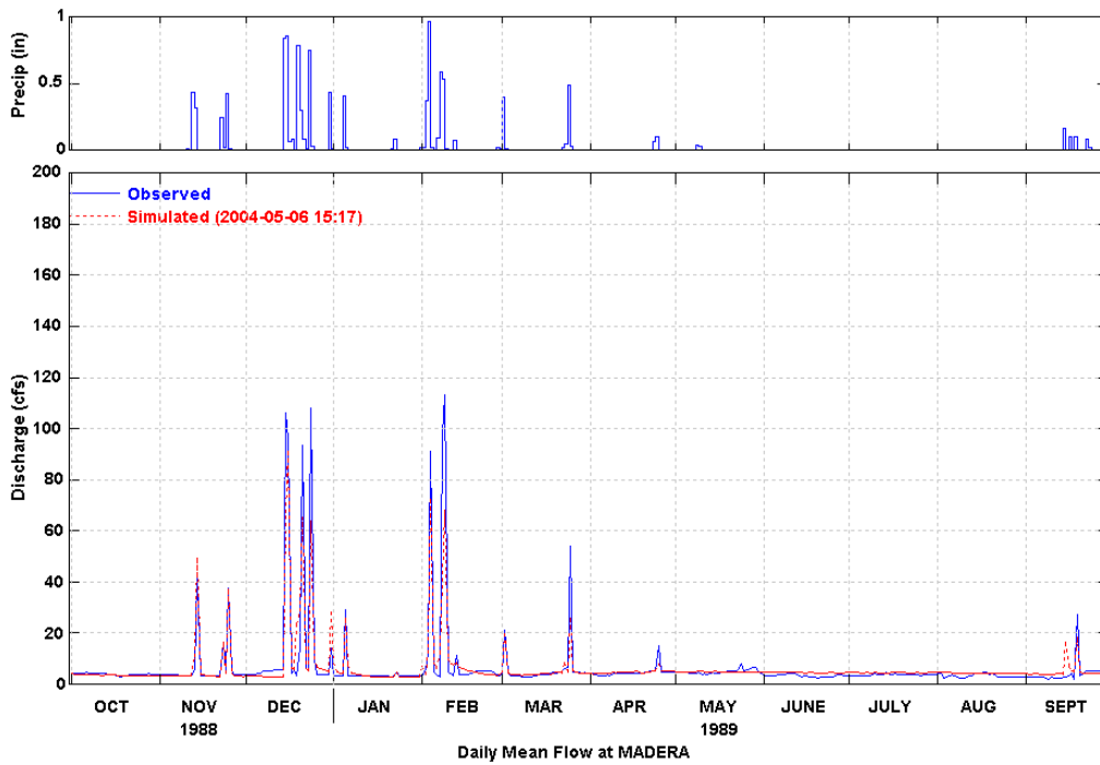
Figure 27 Simulated and Observed Daily Flow at Madera (WY 1989)
