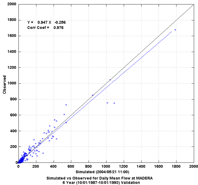
Figure 22 Daily Scatter Plot of Simulated versus Observed Flow at Madera
