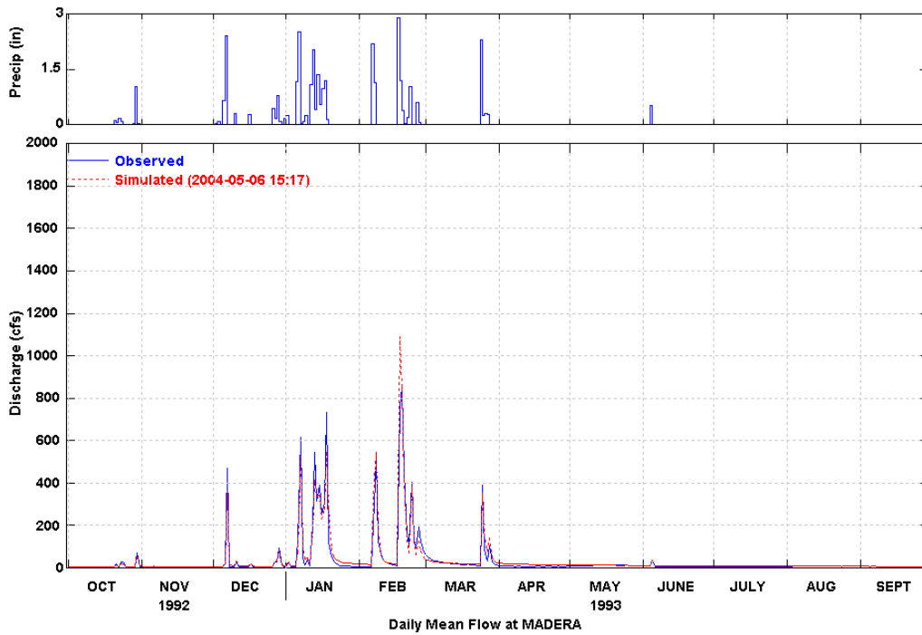
Figure 31 Simulated and Observed Daily Flow at Madera (WY 1993)
