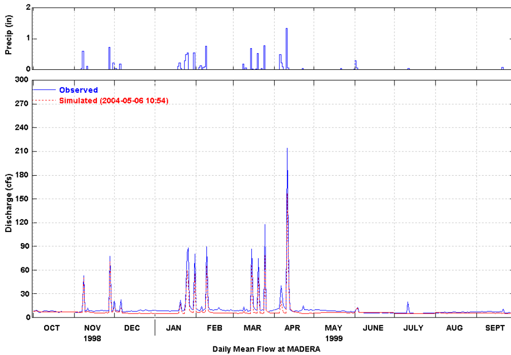
Figure 11 Simulated and Observed Daily Flow at Madera (WY 1999)
