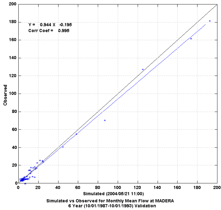
Figure 23 Monthly Scatter Plot of Simulated versus Observed Flow at Madera
