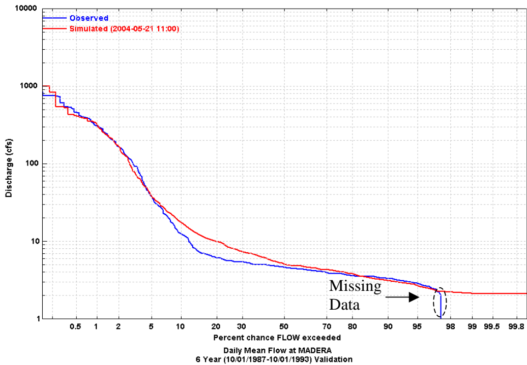
Figure 21 Simulated and Observed Daily Flow Duration Curve at Madera
