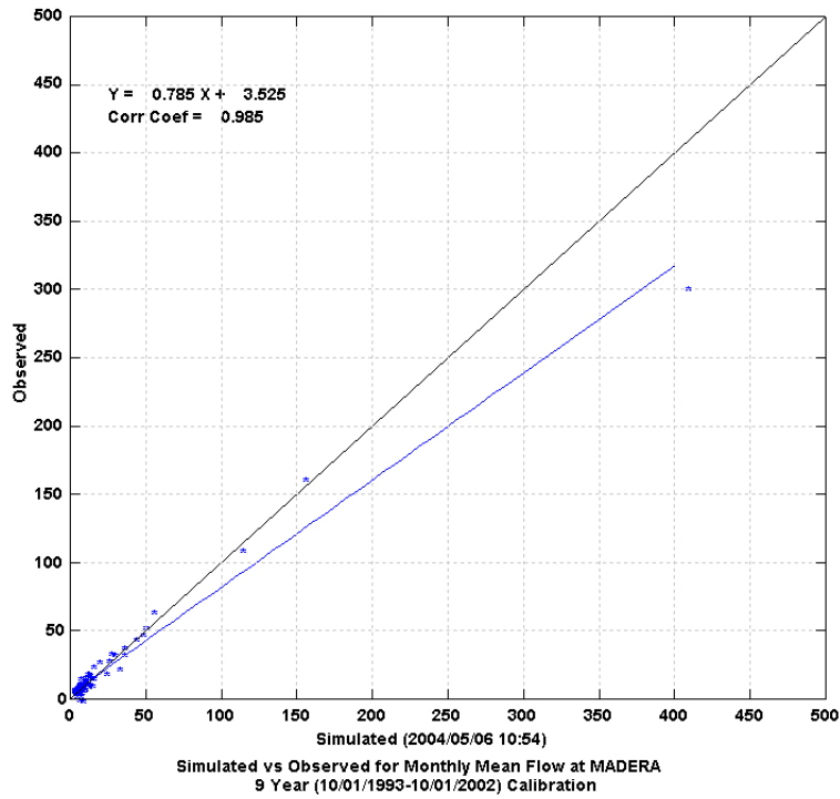
Figure 3 Monthly Scatter Plot of Simulated versus Observed Flow at Madera
