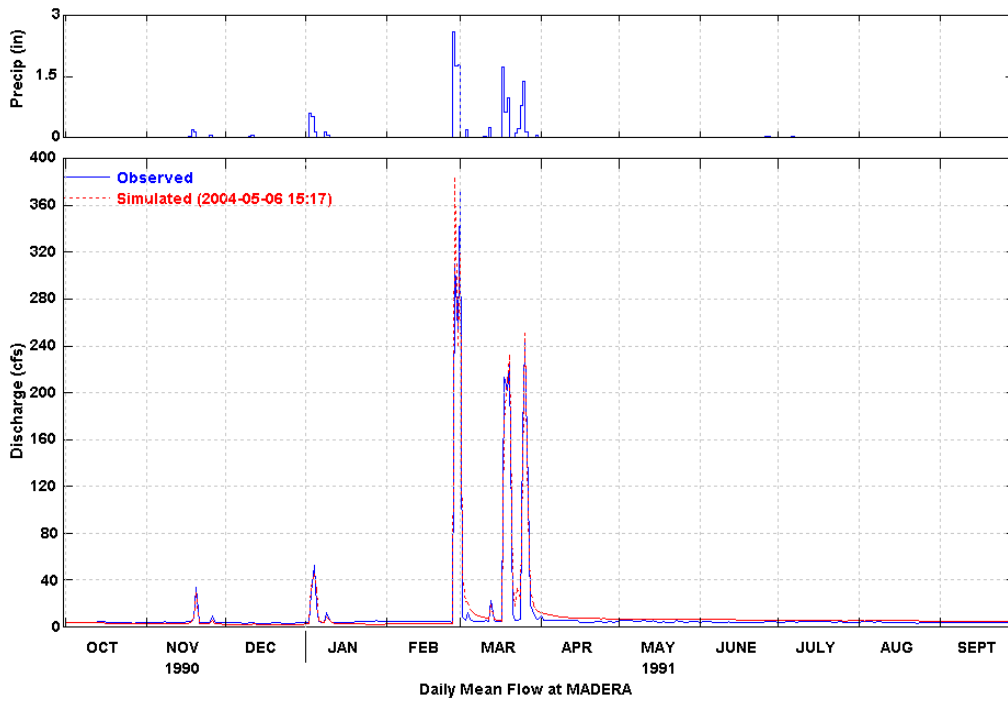
Figure 29 Simulated and Observed Daily Flow at Madera (WY 1991)
