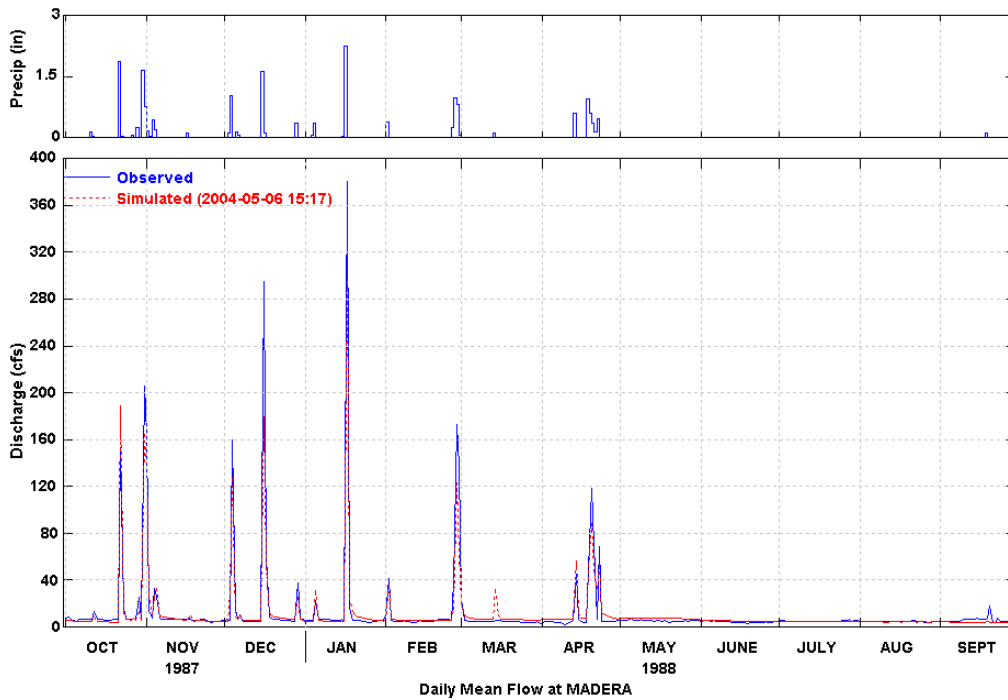
Figure 26 Simulated and Observed Daily Flow at Madera (WY 1988)
