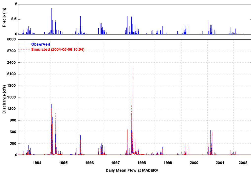
Figure 4 Simulated and Observed Daily Flow at Madera (WY 1994-2002)
