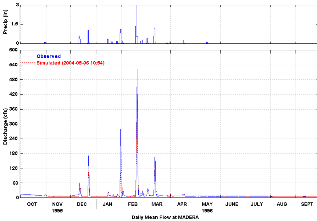
Figure 8 Simulated and Observed Daily Flow at Madera (WY 1996)
