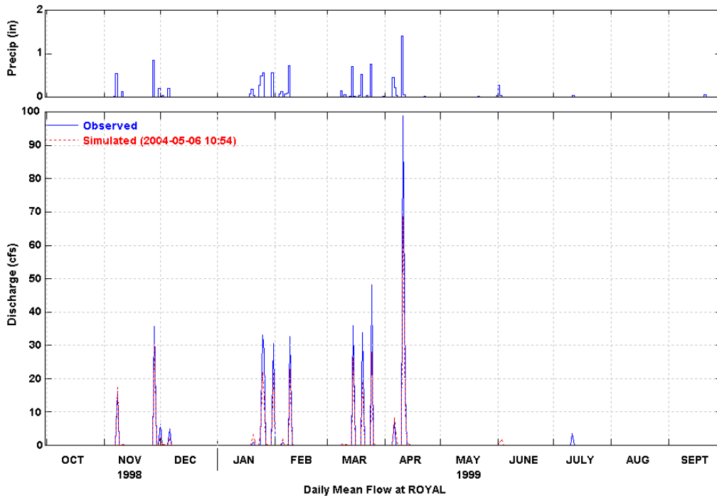
Figure 11 Simulated and Observed Daily Flow at Royal (WY 1999)
