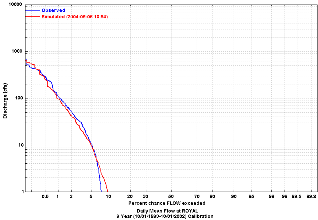
Figure 1 Simulated and Observed Daily Flow Duration Curve at Royal
