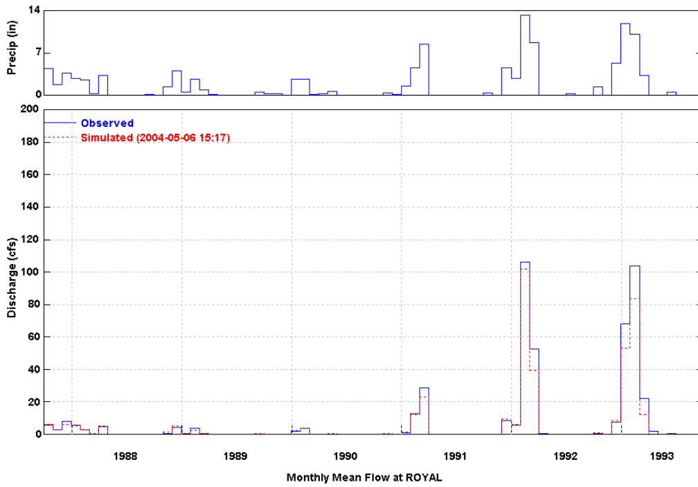
Figure 25 Simulated and Observed Daily Flow at Royal (WY 1988-1993)
