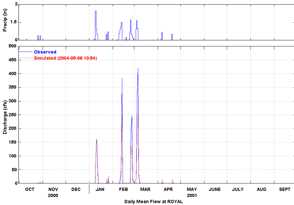
Figure 13 Simulated and Observed Daily Flow at Royal (WY 2001)
