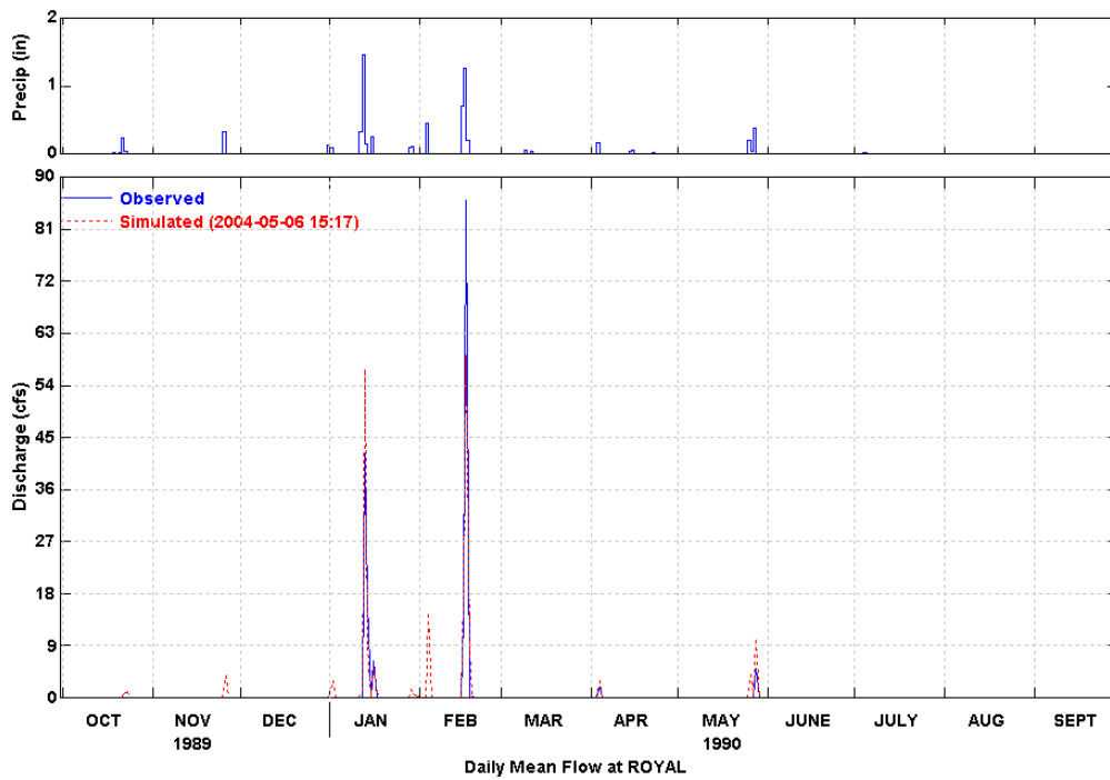
Figure 28 Simulated and Observed Daily Flow at Royal (WY 1990)
