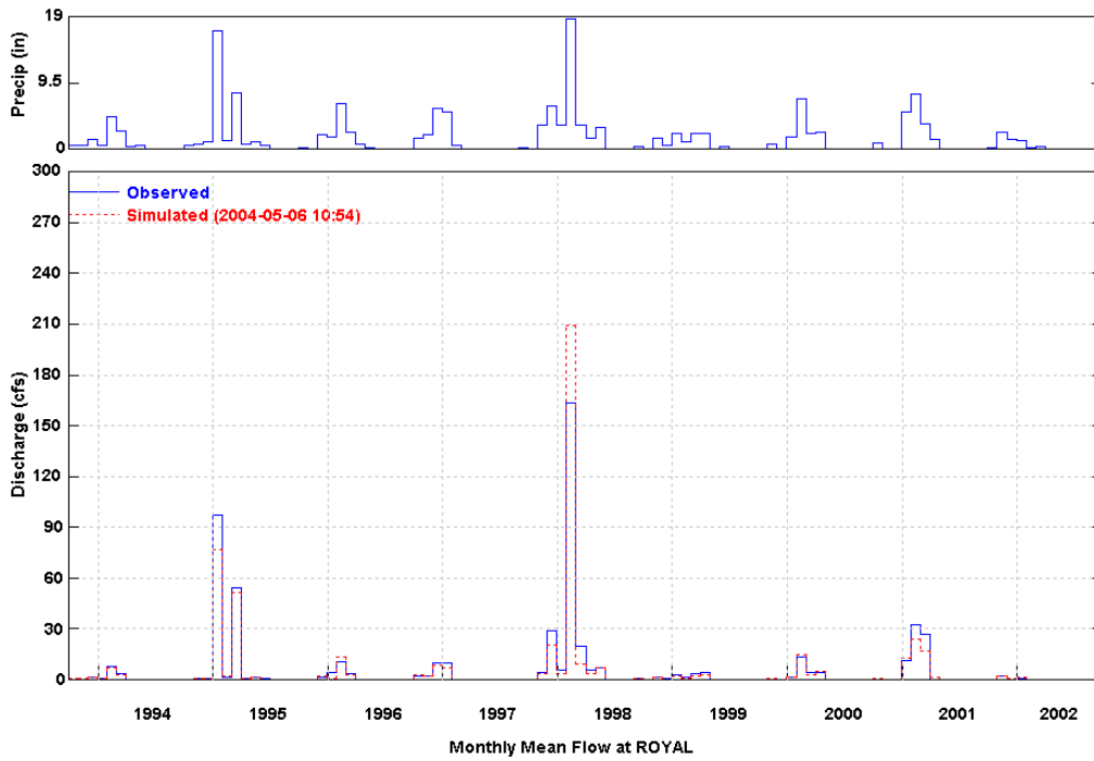
Figure 5 Simulated and Observed Monthly Flow at Royal (WY 1994-2002)
