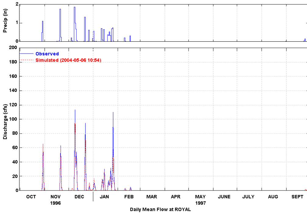
Figure 9 Simulated and Observed Daily Flow at Royal (WY 1997)
