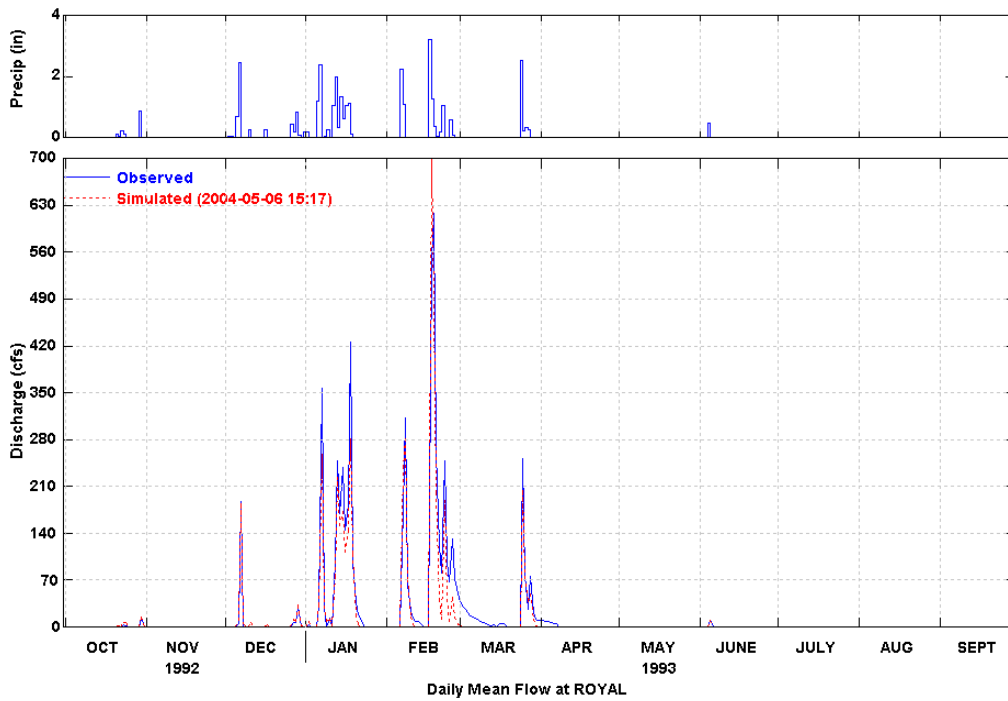
Figure 31 Simulated and Observed Daily Flow at Royal (WY 1993)
