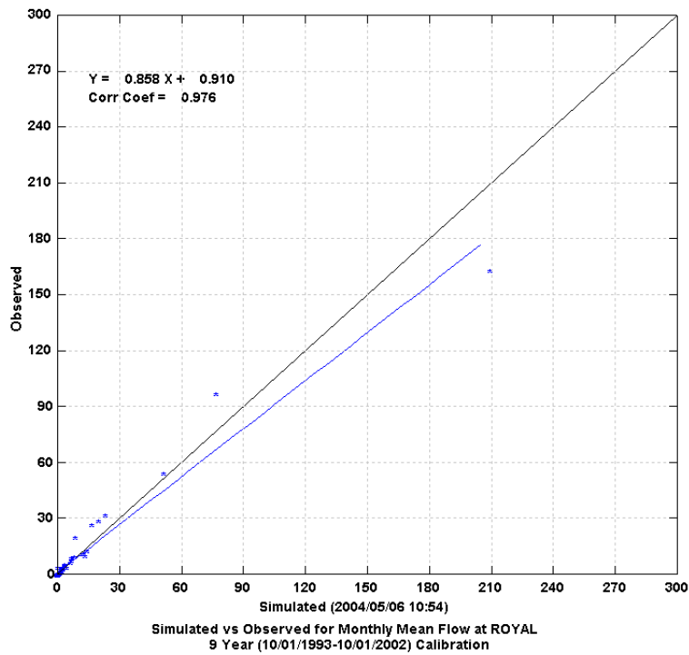
Figure 3 Monthly Scatter Plot of Simulated versus Observed Flow at Royal
