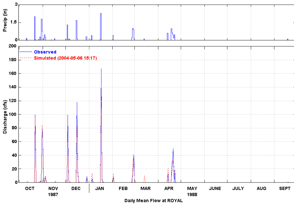
Figure 26 Simulated and Observed Daily Flow at Royal (WY 1988)
