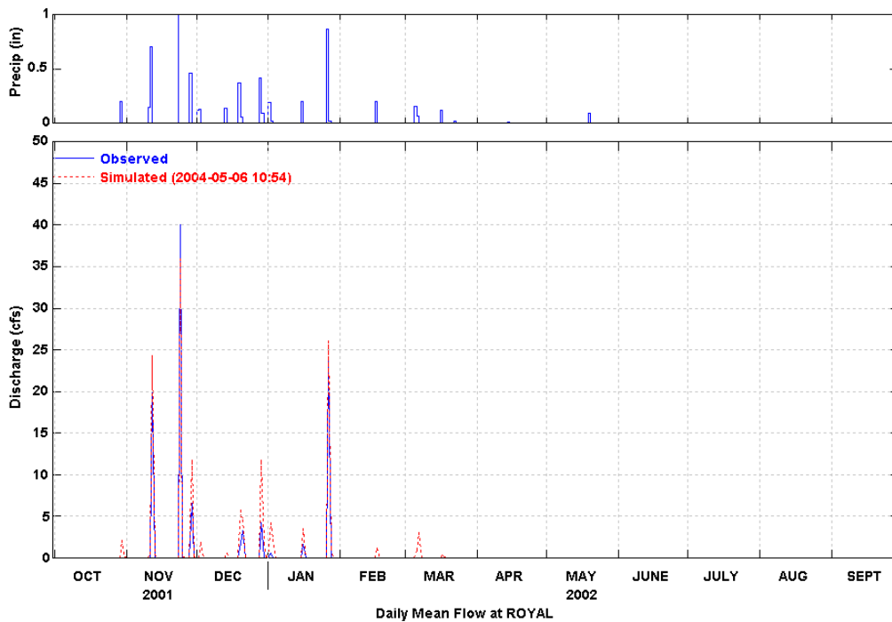
Figure 14 Simulated and Observed Daily Flow at Royal (WY 2002)
