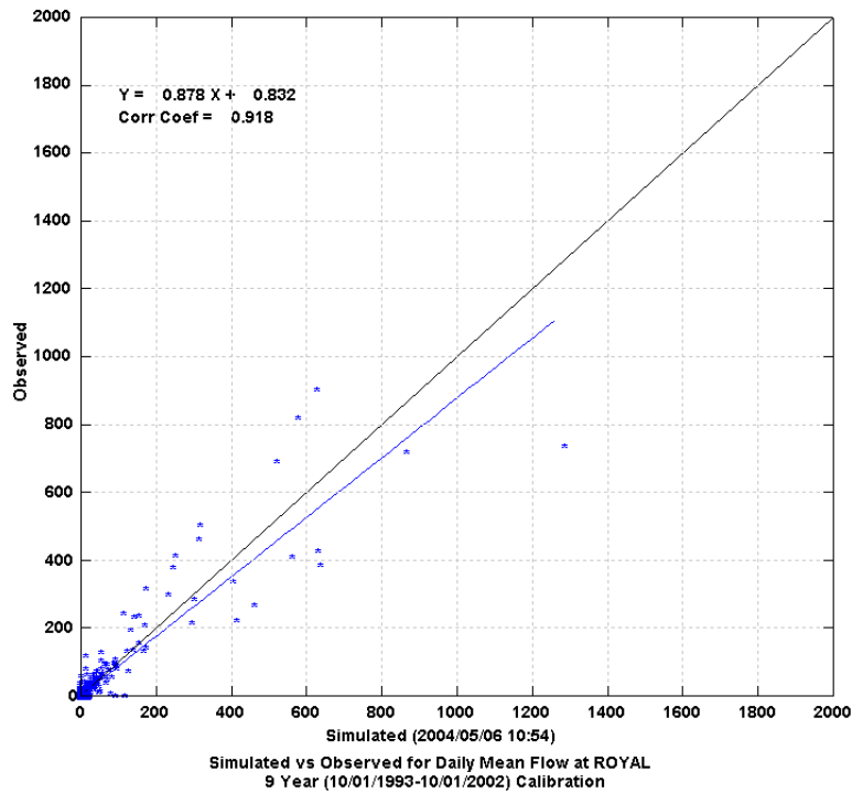
Figure 2 Daily Scatter Plot of Simulated versus Observed Flow at Royal
