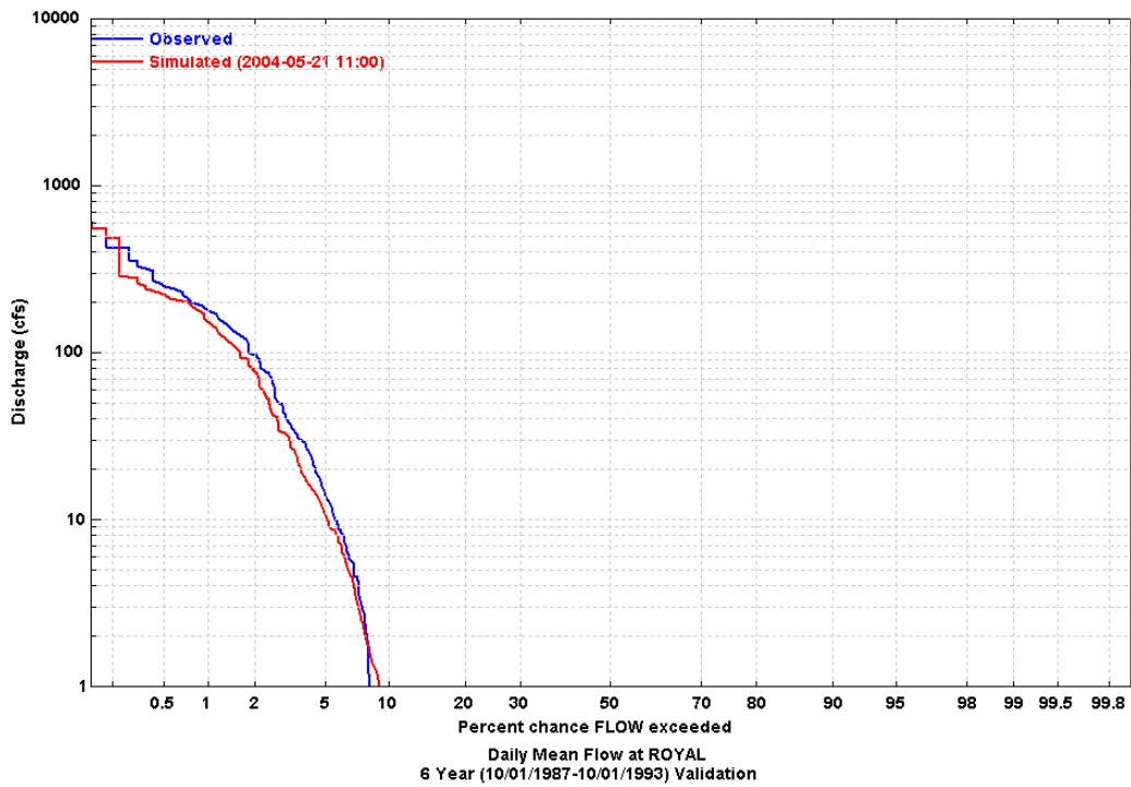
Figure 21 Simulated and Observed Daily Flow Duration Curve at Royal
