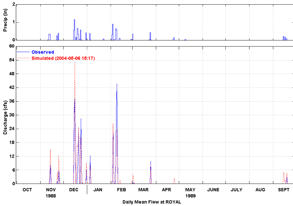
Figure 27 Simulated and Observed Daily Flow at Royal (WY 1989)
