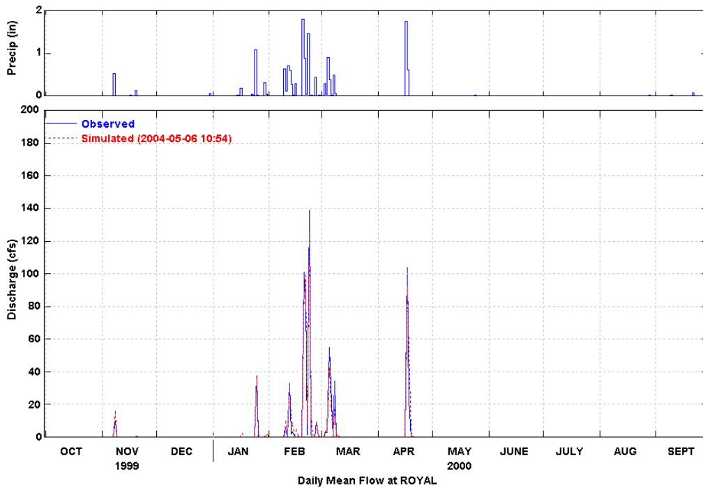
Figure 12 Simulated and Observed Daily Flow at Royal (WY 2000)
