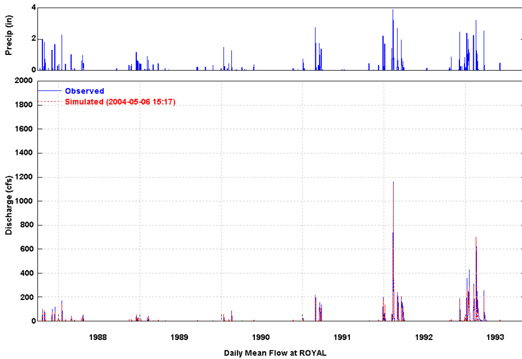
Figure 24 Simulated and Observed Daily Flow at Royal (WY 1988-1993)
