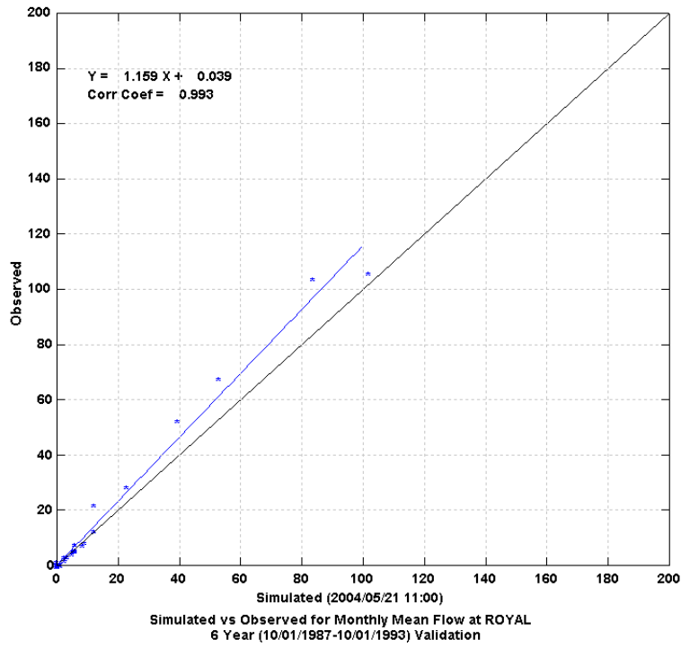
Figure 23 Monthly Scatter Plot of Simulated versus Observed Flow at Royal
