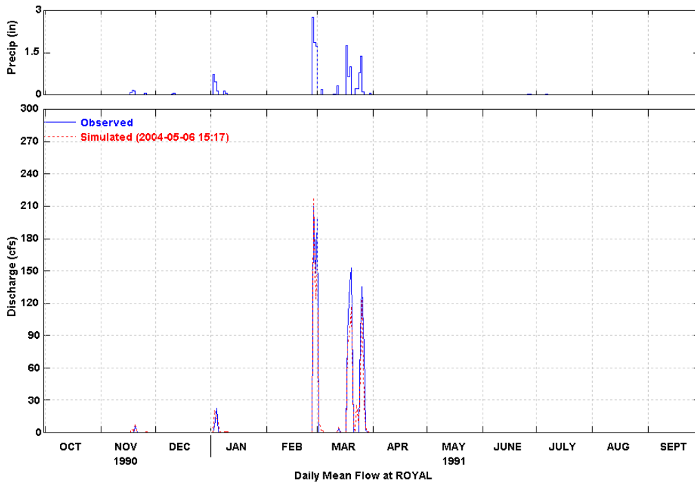
Figure 29 Simulated and Observed Daily Flow at Royal (WY 1991)
