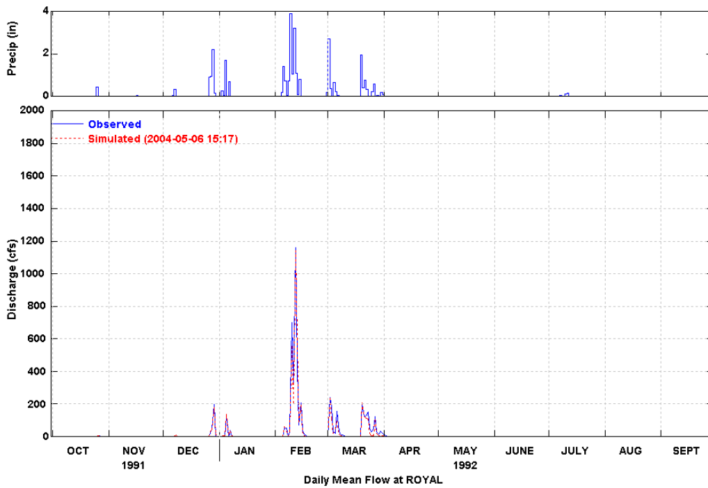
Figure 30 Simulated and Observed Daily Flow at Royal (WY 1992)
