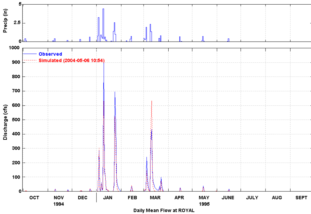
Figure 7 Simulated and Observed Daily Flow at Royal (WY 1995)
